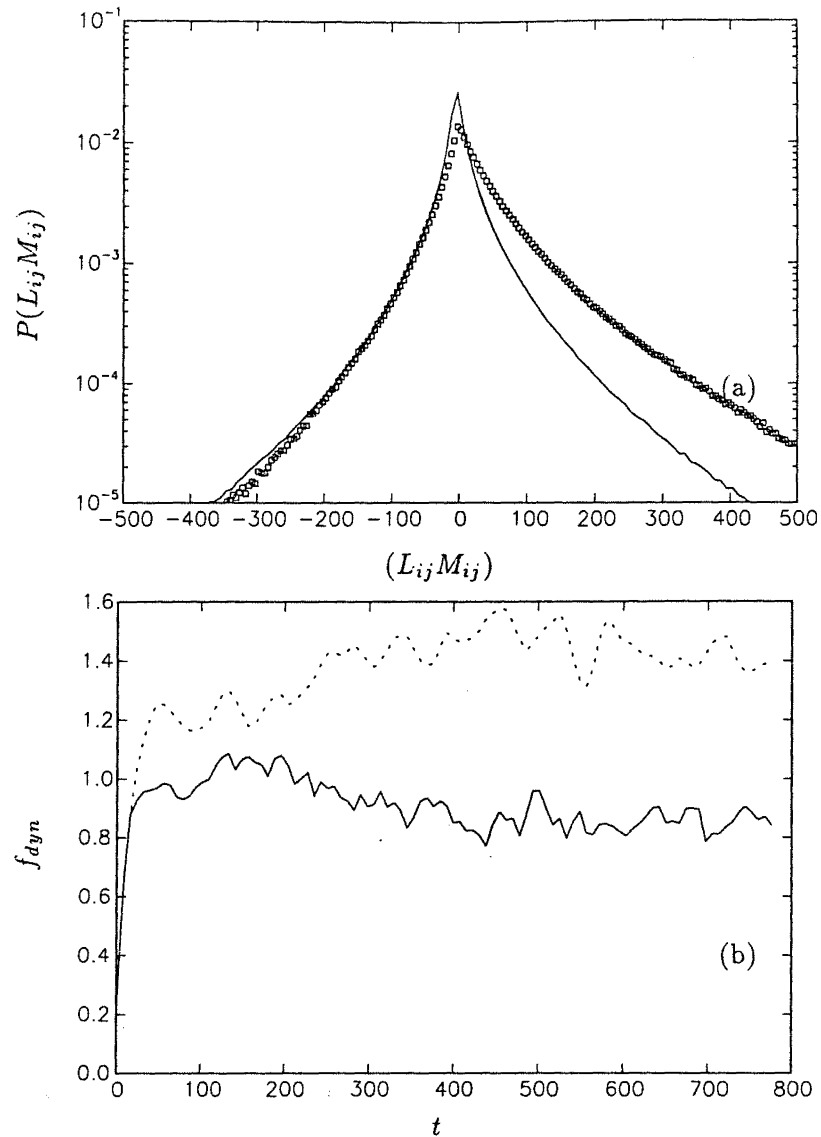
FIGURE 6. (a) PDF of L_{ij}M_{ij} computed with same grid but different test filters. Both statistics were performed on the same fields simulated on a 128 \times 128 \times 16 grid and with test filter cutting off at \bar{k}_i = 1/2\bar{k}_i . The solid line refers to L_{ij}M_{ij} computed as in the simulation, while the symbols refer to L_{ij}M_{ij} computed with a test filter cutting off at \bar{k}_i = 1/2\bar{k}_3 . (b) anisotropy factor f_{dyn} computed with an anisotropic test filter (—) and with an isotropic (larger scale) test filter (.....). The predicted value is 1.34.
