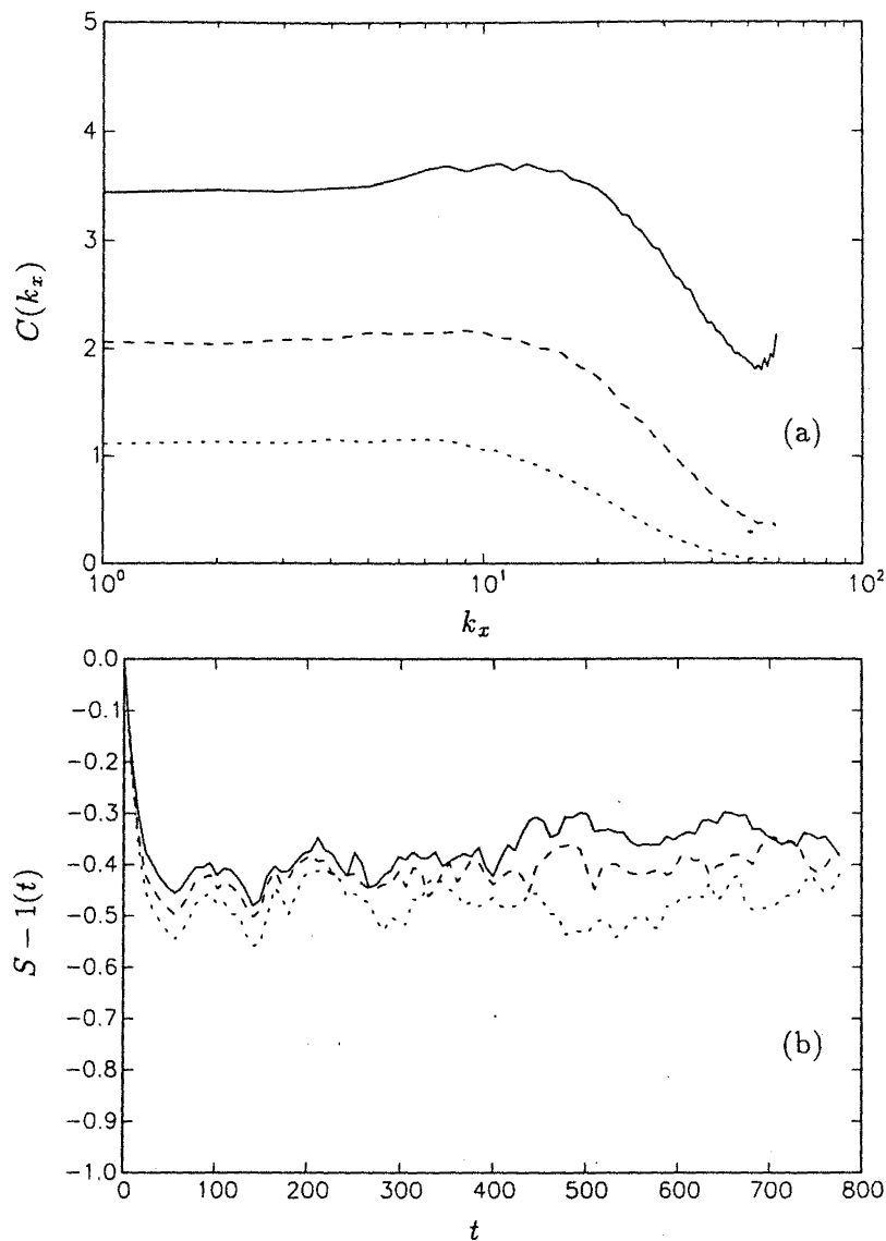
FIGURE 5. Pencil-like grid. (a) compensated 1-D spectrum: dynamic model (—), modified Smagorinsky (.....) and Smagorinsky-Deardoff (----). (b) derivative skewness in the best resolved direction, same symbols as above.
