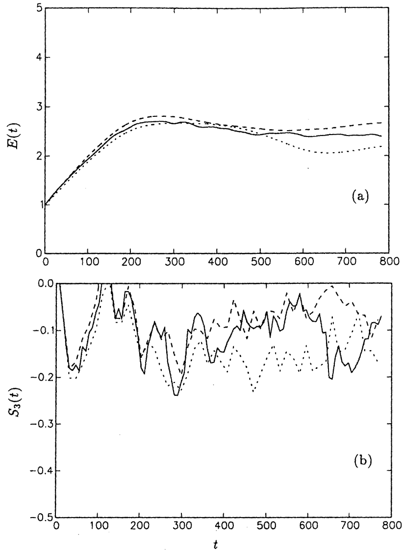
FIGURE 2. Eddy-viscosity models on pancake-like grids ( 256 \times 16 \times 16 ). (a) kinetic energy as a function of time for dynamic model (—), modified Smagorinsky (.....), and Smagorinsky-Deardoff (---). (b) skewness in the worst resolved direction, same symbols as in (a).
