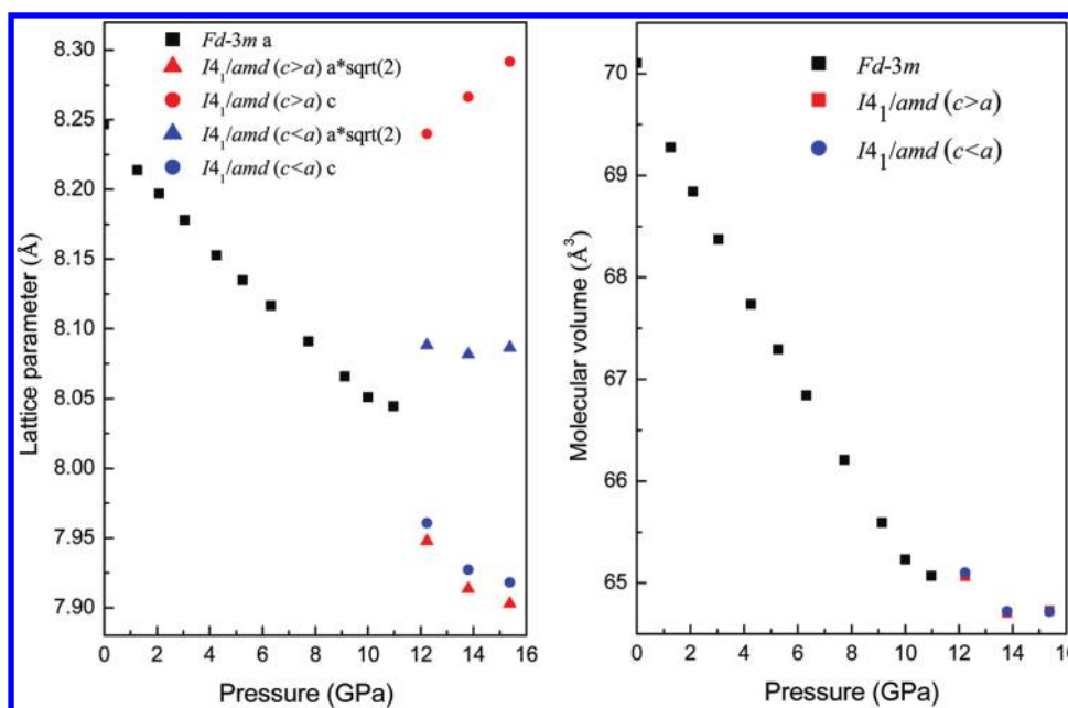
Figure 2. Development of lattice parameters and volume per molecule in the spinel structure and the distorted tetragonal phases of bulk \text{LiMn}_2\text{O}_4 as a function of pressure. The a\sqrt{2} is used in tetragonal phases for straightforward comparison between the undistorted and distorted cubic structures.
