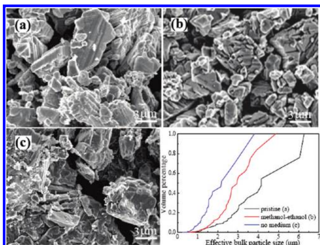
Figure 4. SEM images of (a) pristine commercial \text{LiMn}_2\text{O}_4 powder, (b) bulk samples after compression in a mixture of methanol–ethanol, and (c) the quenched bulk samples after compression without pressure medium. Statistical analysis of images (a)–(c) shows the accumulation of volume percentage as a function of the particle size.
