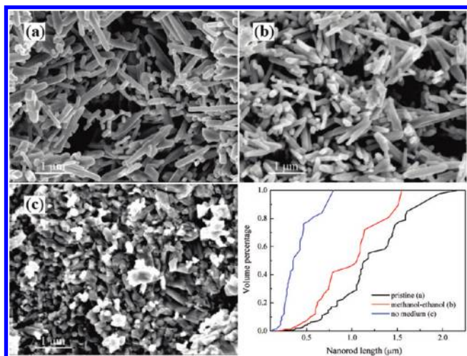
Figure 7. SEM images of (a) well-characterized pristine \text{LiMn}_2\text{O}_4 nanorods before compression, (b) quenched nanorods after compression in a mixture of methanol–ethanol, and (c) after compression without pressure medium. Statistical analysis of images (a)–(c) showing the accumulation of volume percentage as a function of nanorod length quantifies the significant morphology change between the nanorods under nonhydrostatic conditions and the pristine nanorods as well as those quenched from hydrostatic compression.
