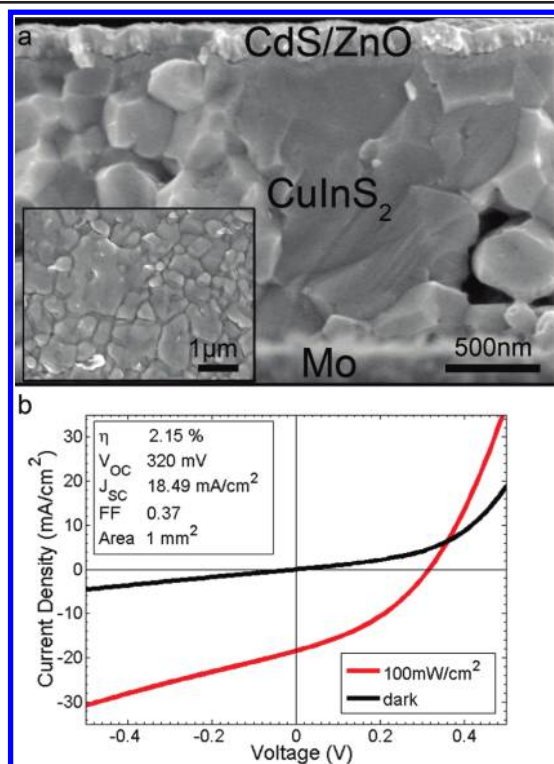
Figure 2. (a) SEM cross section of a solar cell. Inset: top view of the \text{CuInS}_2 film. (b) \text{CuInS}_2 solar cell characteristics.
