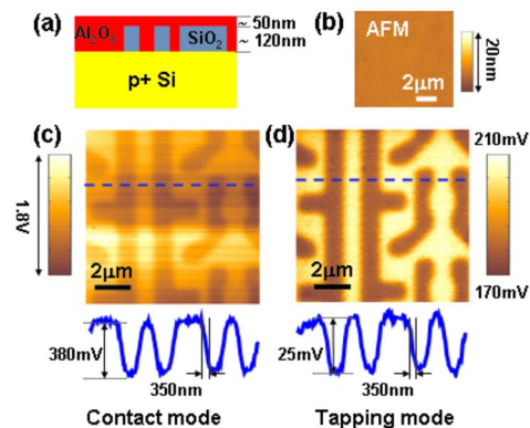
FIG. 3. (Color online) (a) Layer structure of the \text{Al}_2\text{O}_3 – \text{SiO}_2 /Si sample. (b) AFM image of the polished sample surface. (c) Contact and (d) tapping mode MIM-C images taken by the same tip at the same area. The darker regions are buried \text{SiO}_2 . Electronic drift can be observed in (c) but not in (d). Line cuts are shown in both (c) and (d) for comparisons of the signal strength and the spatial resolution.
