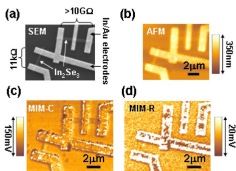
FIG. 4. (Color online) (a) SEM picture of \text{In}_2\text{Se}_3 nanoribbons and In/Au electrodes. The tapping data on the same devices are shown as (b) topography, (c) MIM-C, and (d) MIM-R images. The lower left device is more conductive than the one in the upper right.
