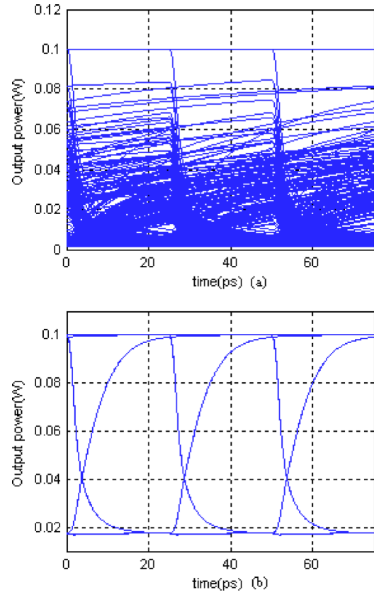
FIG. 7. The eye diagrams for a non-return-to-zero optical link at 40 Gbps: (a) with no boundary conditions and (b) with V=0 boundary condition. Similarly, the V=0 boundary condition significantly improves the eye diagrams.
