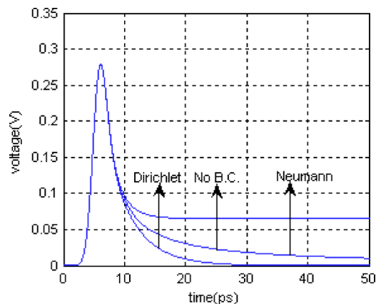
FIG. 4. Total voltage change for the three different boundary conditions (no boundary, V=0 , and \nabla V=0 ) at the center of the switch.
