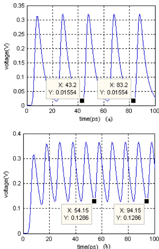
FIG. 5. Steady state behavior of a pulse train having a period of (a) 20 and (b) 10 ps. It is clear that both pulse trains reach steady state. When the period is smaller, the device reaches the steady state later and at a higher steady state value.
