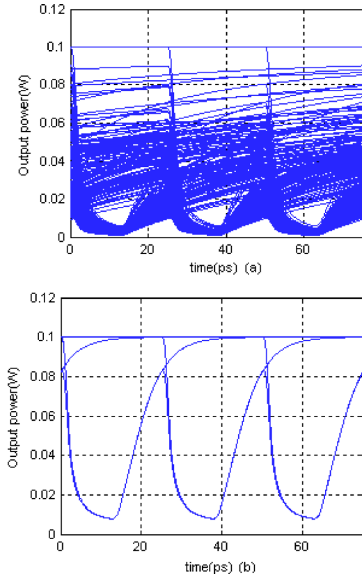
FIG. 6. The eye diagrams for a return-to-zero (RZ) optical link at 40 Gbps: (a) with no boundary conditions and (b) with V=0 boundary condition. The improvement resulting from the V=0 boundary condition is clearly evident on the opening of the eye diagrams.
