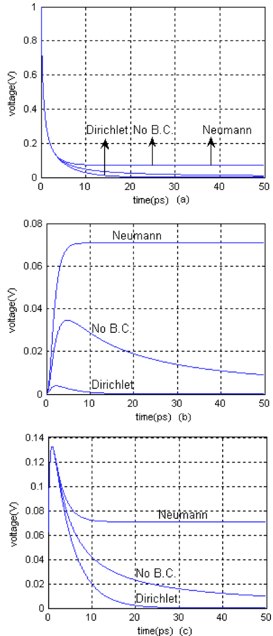
FIG. 3. Diffusive conductive voltage decay due to the three different boundary conditions (no boundary, V=0 , and \nabla V=0 ): (a) at the center of the switch, (b) at a point very near to the switch contact line, and (c) at the midpoint between the switch center and contact.
