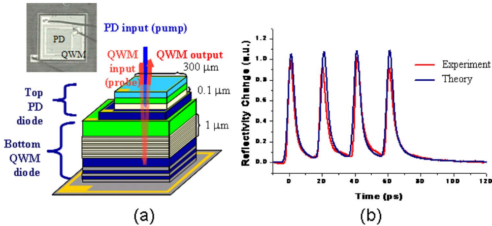
FIG. 1. (a) Architecture of a vertically integrated double-diode optoelectronic switch based on diffusive conduction, with an inset of a plan-view micrograph of the fabricated switch and (b) the 50 GHz experimental operation of the switch along with our theoretical simulation.
