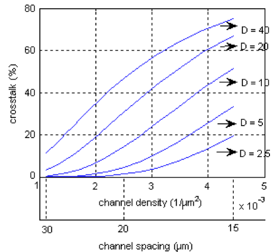
FIG. 8. Multichannel operation. The crosstalk is plotted as a function of channel spacing (and channel density) for different device diffusive constants D (in \mu\text{m}^2/\text{ps} ).
