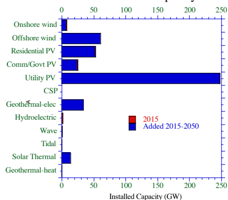
Figure 3. 2015 and proposed 2015-2050 additions of installed capacity of WWS generators for Taiwan.
