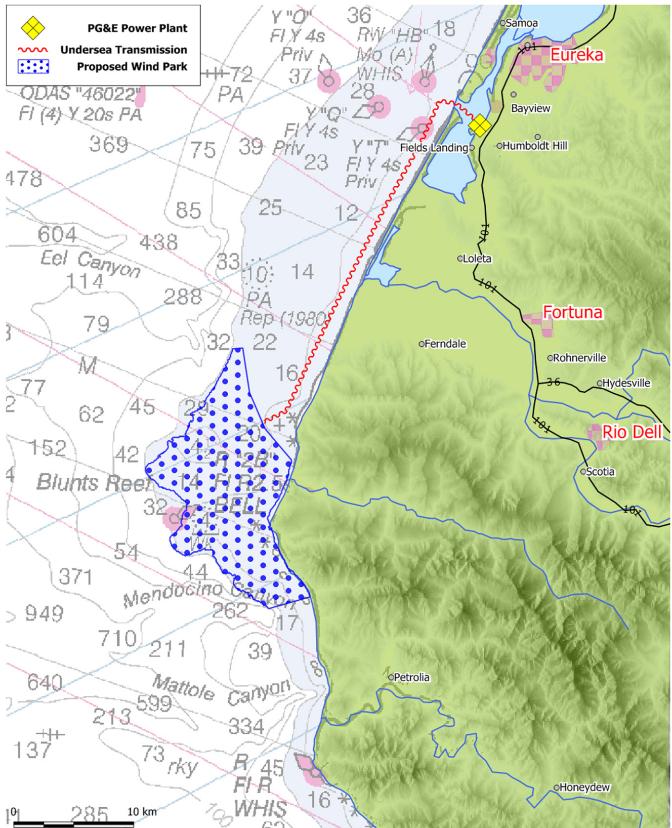
Fig. 4. A proposed wind farm off the Coast of Cape Mendocino located in water shallow enough for multi-leg turbine foundations ( \leq 50 m) and having annual \bar{v}_{80\text{ m}} \geq 7.5 \text{ms}^{-1} (based on the 2005/2006 model data). An undersea transmission cable would connect the wind farm to an existing power plant location in Humboldt Bay.
