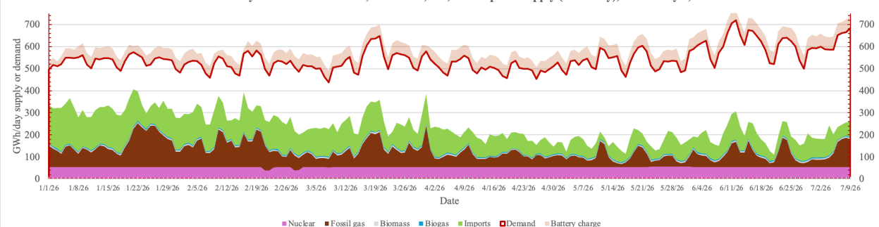
CAISO Grid Daily Demand and Nuclear, Fossil Gas, Bio, and Imports Supply (GWh/day), Jan. 1-July 9, 2026
