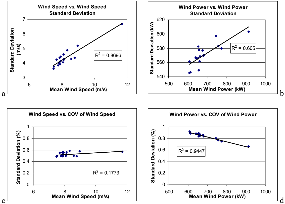
Figure 6 Standard deviations and coefficients of variation of wind speed and wind power at the 19 sites selected.
