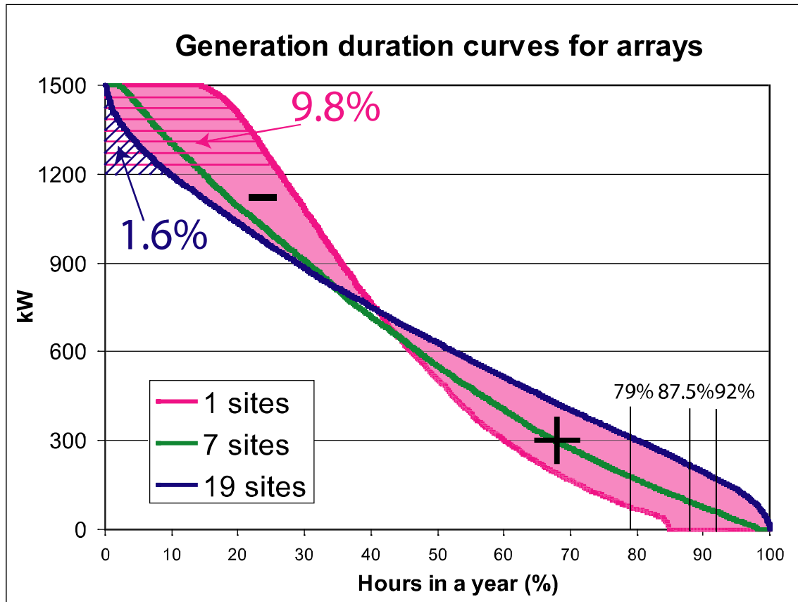
Figure 3 Generation duration curves for base-case array configurations: single-, 7-, and 19-site arrays. Each point on the x-axis represents the percent of hours in a year that wind power production is greater than or equal to the corresponding power (y-axis) on the curve. The area below the generation curve represents the total energy (kWh) produced in a year by the array. Shaded areas are described in the text. The thatched areas are the energy lost (9.8% and 1.6%) if the size of transmission lines is reduced from 1500 kW to 1200 kW for the 1- and 19-site arrays, respectively.
