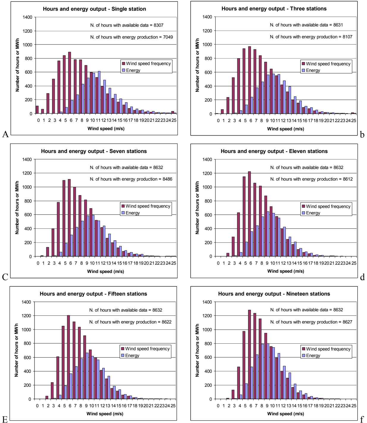
Figure 5 Number of hours and energy output (kWh) at given wind speeds (m/s) for all hours of the year 2000 averaged over: (a) one, (b) three, (c) seven, (d) 11, (e) 15, and (f) 19 stations.
