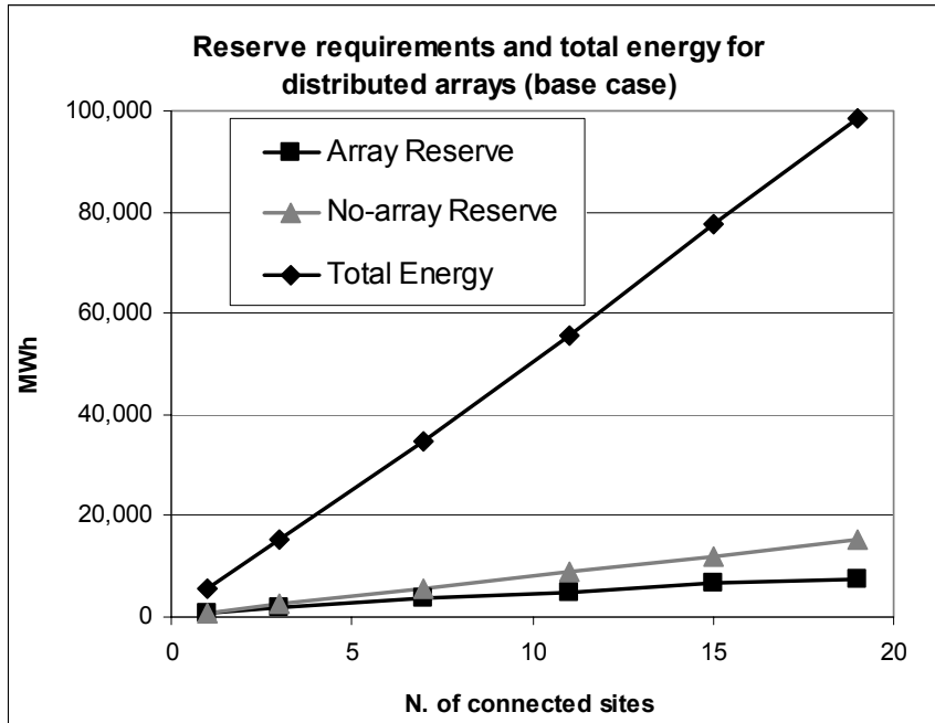
Figure 8 Reserve requirements in a year (MWh) for the base array and for the no-array cases (sites if they were not interconnected). Total energy (MWh) produced by the array in a year is also shown.
