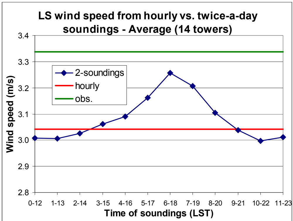
Figure 10 Observed, calculated from hourly V_{ref} , and calculated from daily averages of V_{ref} with twice-a-day soundings values of LS wind speed, averaged over all two-level towers of the KSC network.
