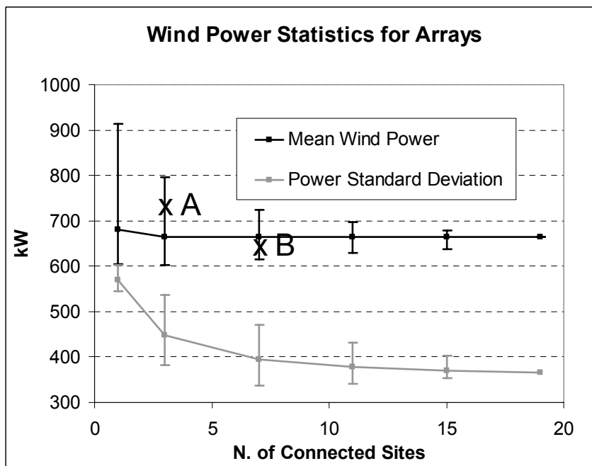
Figure 4 Wind speed (a) and wind power (b) statistics for interconnected arrays as a function of number of connected sites. The bars indicate the range of values obtained from all possible combinations of the given number of connected sites.
