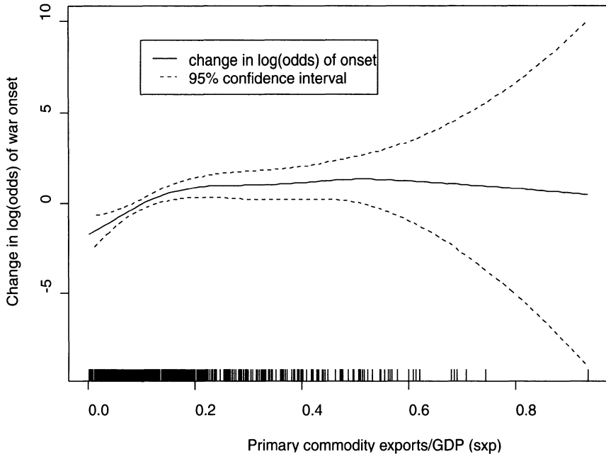
Figure 3: Change in Log(Odds) of Civil War as a Function of sxp
