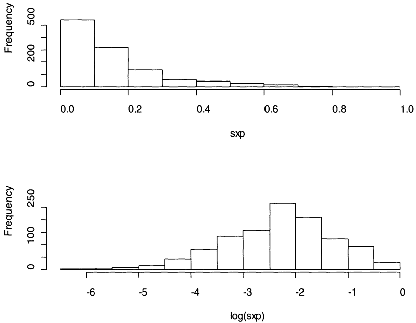
Figure 1: Histograms of sxp and \log(sxp)
