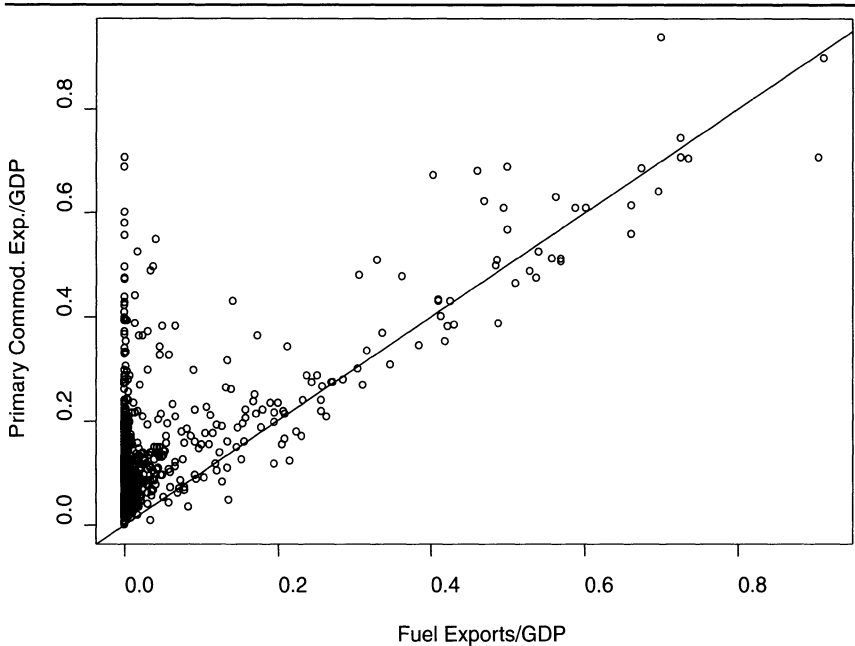
Figure 2: Fuel Exports and sxp
