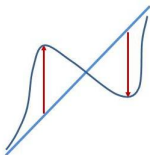
transforming a monotone region into one with a maximum and a minimum
