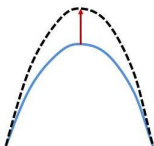
amplifying a maximum
