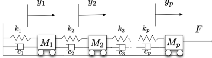
Figure 2. Mass-damper-spring system.
