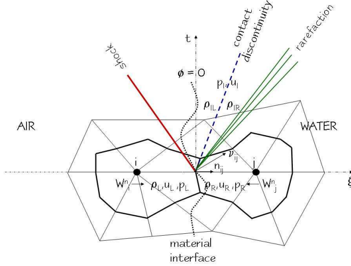
Fig. 2. Illustration of the local, one-dimensional, two-phase Riemann problem on a two-dimensional grid. (Subscripts I , L , and R denote the material interface and the media at its left and right sides, respectively. n_{ij} denotes the normal to the control volume at the face between nodes i and j . \nu_{ij} denotes the normal to the material interface at the same point).
