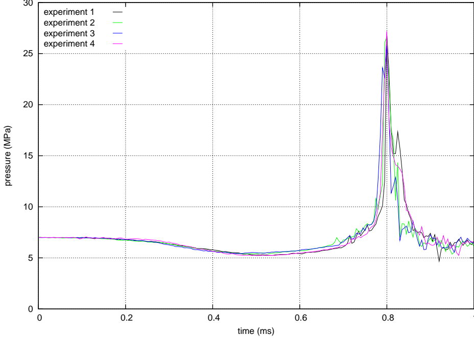
Fig. 9. Pressure time-histories recorded at one of the sensors during the four experiments described in [27].
