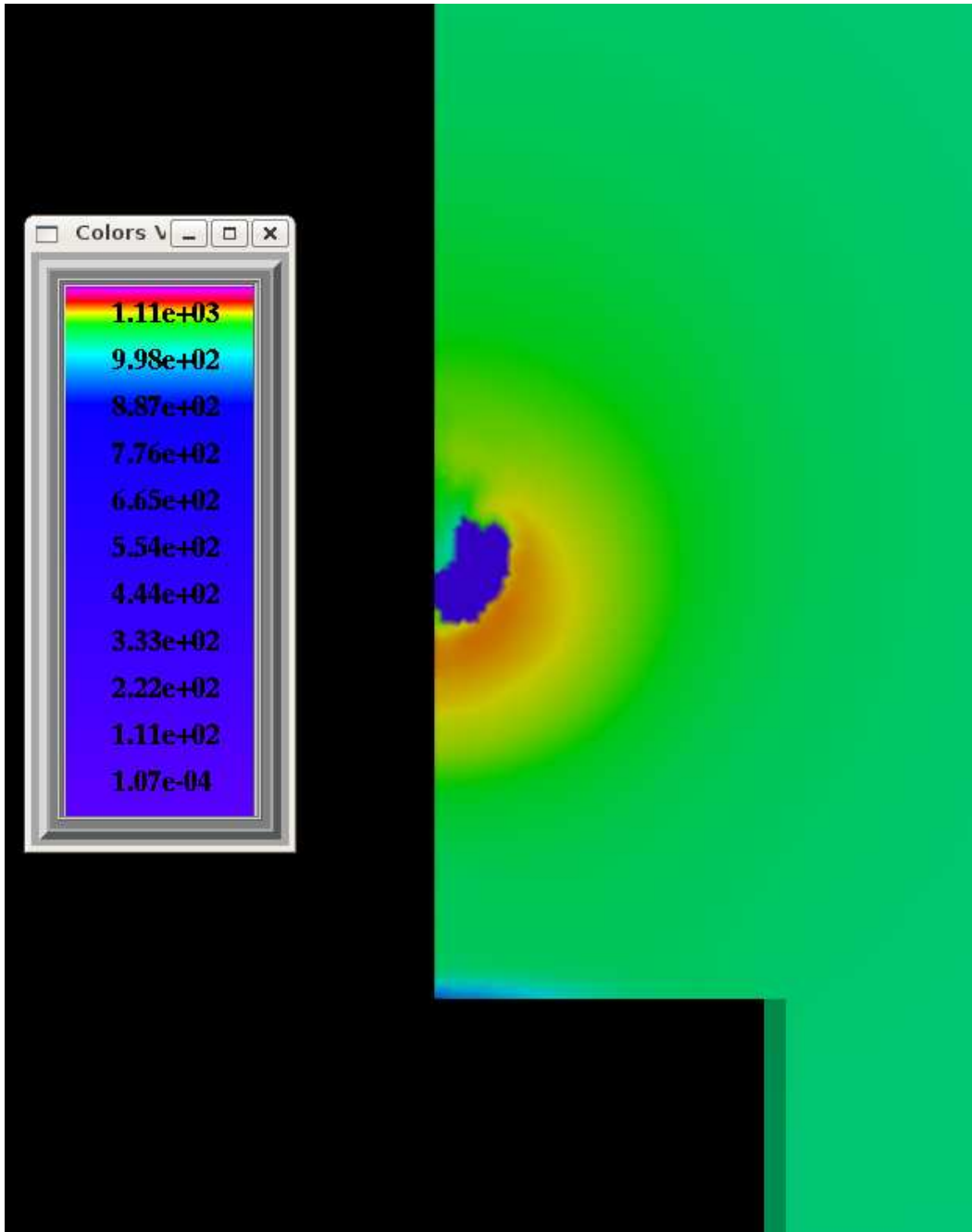
Fig. 11. Density contourplots (in \text{kg}/\text{m}^3 ) predicted by AERO-F equipped with the GFMP-ERS in the vicinity of the air bubble during its collapse.
