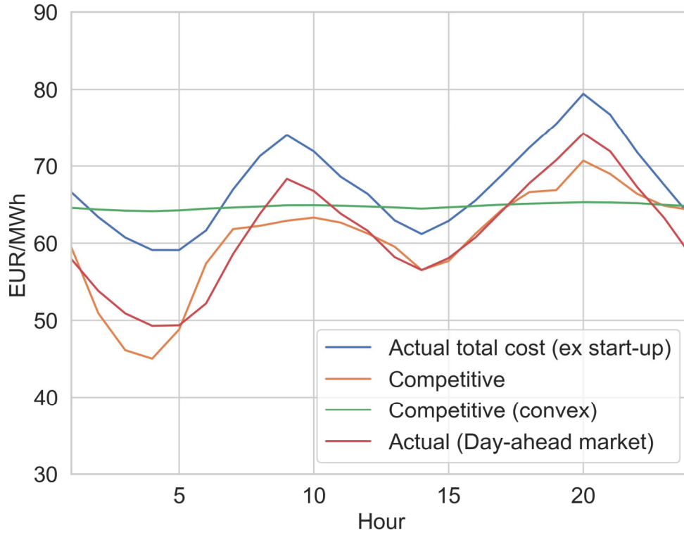
Figure 6: Competitive Benchmarks
