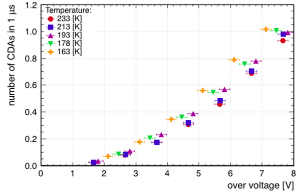
Fig. 13. Number of Correlated Delayed Avalanches (CDAs) per primary pulse within a time window of 1 \mu s after the trigger pulse as a function of the applied over voltage for different SiPM temperatures.
