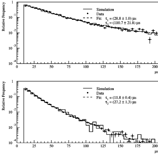
FIG. 1. Top: the distribution of time between muon hits and the single-neutron capture events, fitted to the exponential function, Eq. (3). Bottom: the distribution of time between muon hits and the first neutron capture events for the double-neutron events with an exponential fit, Eq. (3). In both panels the Monte Carlo simulation is shown as a histogram, and the fitted time constants \tau_1 and \tau_2 are displayed.
