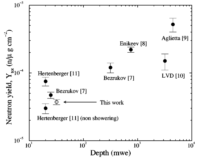
FIG. 3. Summary of available data on the total neutron yield Y_{tot} versus depth. The points are labeled by the corresponding first author. For Ref. [11] two results are shown, with and without the effect of external showers. Present work is denoted by an open circle.
