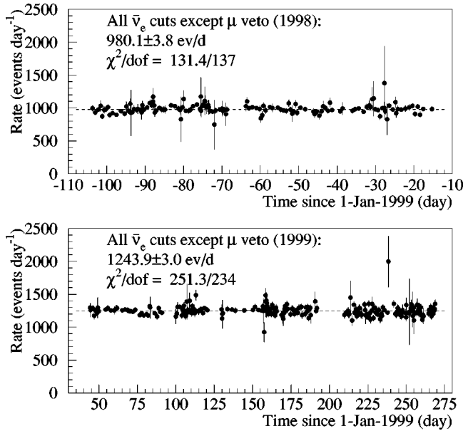
FIG. 19. The number of candidates per day in the 373 runs used in this analysis, fit to a constant for each year. All neutrino selections except the previous muon time cut are used, leaving a data set dominated by muon-induced neutron background. The different rates in 1998 and 1999 are due to trigger and livetime improvements.
