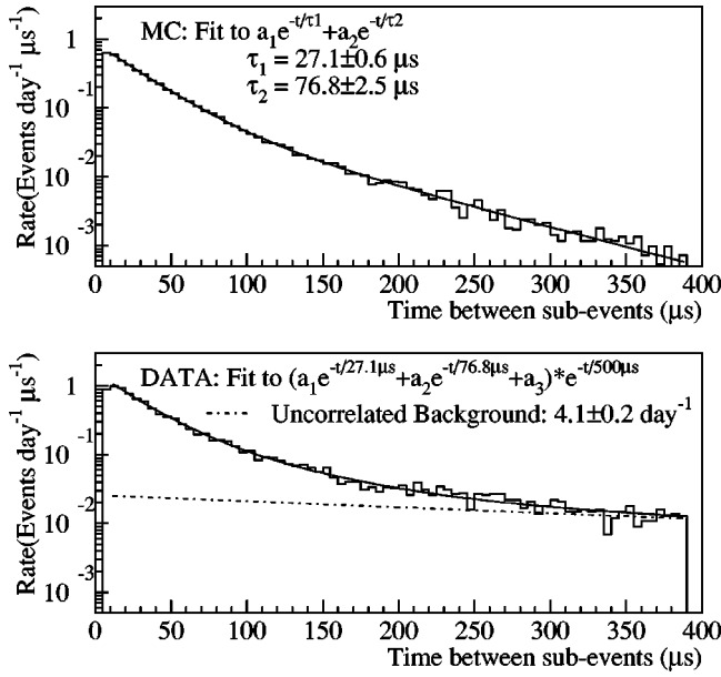
FIG. 15. The time elapsed between the prompt and delayed portion of neutrino candidate events for Monte Carlo simulation and data. The Monte Carlo simulation is fit to two exponentials. The data are fit to three exponentials, constrained to have the time structure of the simulation and an additional contribution due to uncorrelated background (dashed line).
