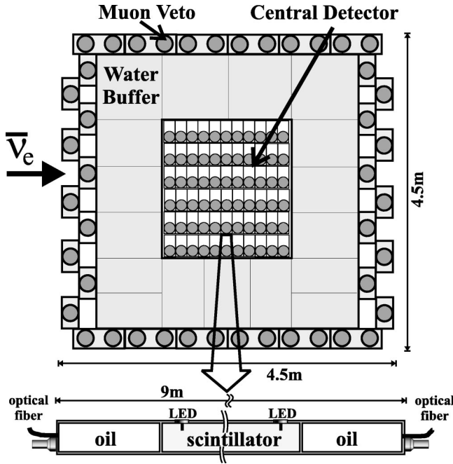
FIG. 1. The Palo Verde detector. One of the 66 target cells with PMTs, calibration light emitting diodes (LEDs), and optical fiber flashers is shown lengthwise at the bottom.
