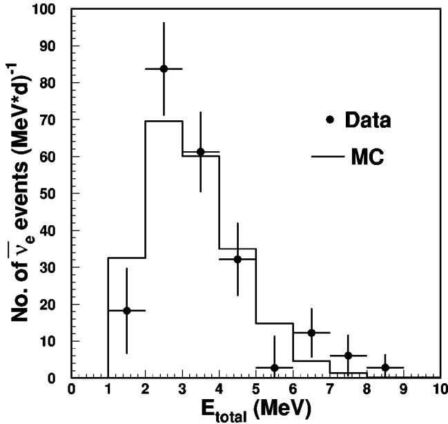
FIG. 22. Total energy of the prompt subevent ( \sim E_{\nu_e}^- - 1.8 MeV) in 1 MeV wide energy bins (observed and expected for no oscillation) from the on-off analysis, summed over 1998 and 1999. The spectra are in agreement with each other, with a \chi^2/N_{\text{DF}} = 8.5/8 . Uncertainties are statistical only.
