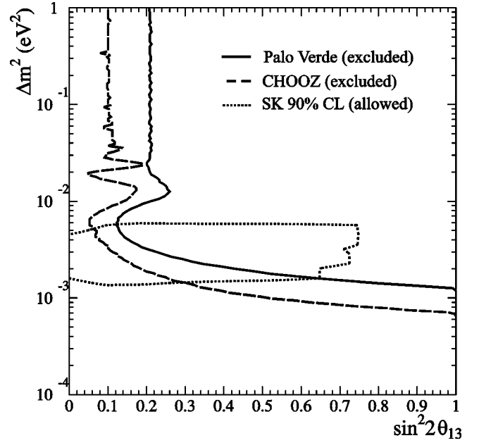
FIG. 24. Exclusion plot showing the allowed region of \theta_{13} and \Delta m^2 based on the Super-Kamiokande preliminary analysis (the region inside the dotted curve). The region excluded by the neutrino reactor experiments are to the right of the corresponding dashed and continuous curves.
