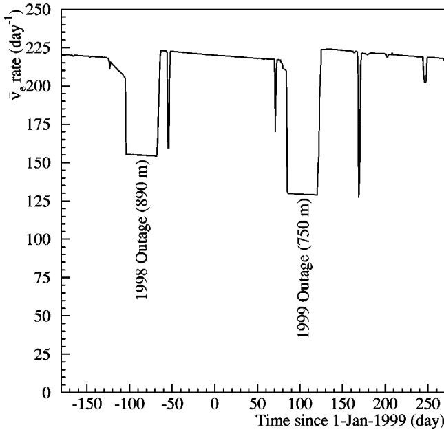
FIG. 4. The calculated \bar{\nu}_e interaction rate in the detector target. The two long periods of reduced flux from reactor refuelings were used for background subtraction. The decreasing rate during the full power operation is a result of the changing core composition as the reactor fuel is burned.
