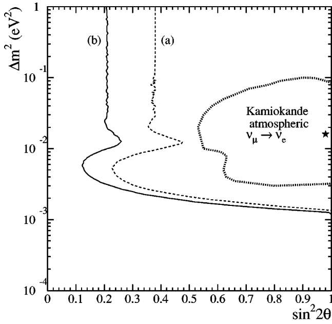
FIG. 23. 90% C.L. limits of oscillation parameters for (a) the reactor power analysis, which fits for background based on varying power levels, and (b) the swap analysis, which directly subtracts background from the data set. The Kamiokande \nu_e - \nu_\mu atmospheric neutrino 90% C.L. (dashed line) and best fit (star) are also shown.
