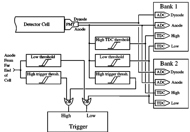
FIG. 2. Schematic of the front-end electronics. The charge and timing of PMT pulses are read out by two banks of ADCs and TDCs. The timing information is discriminated with two thresholds to avoid crosstalk and retain dynamic range. Trigger discriminator signals from the two PMTs in each cell are OR'ed and input to the trigger circuit.
