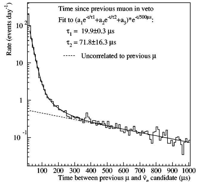
FIG. 18. The time between the previous muon traversing the veto counter and a neutrino candidate event trigger. The fit is to a sum of three exponentials. The dashed portion denotes events uncorrelated to the previous muon; the rest are correlated background events induced by cosmic muons. The neutron capture time constants, shorter than the simulation prediction for \bar{\nu}_e events, imply multiple neutron production.
