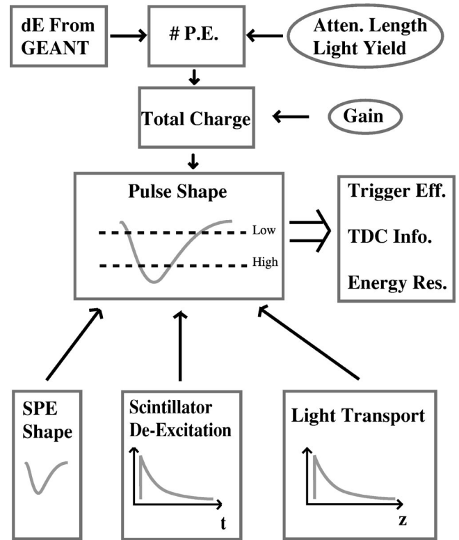
FIG. 8. Schematic of the Monte Carlo detector simulation program. In order to convert energy deposited into accurate threshold simulation, calibration information from the detector was used to reconstruct PMT pulses.
