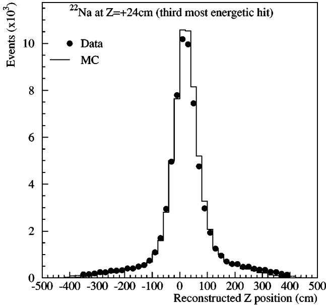
FIG. 10. A comparison of the reconstructed Z position of an annihilation gamma energy deposit from a ^{22}\text{Na} run, between data and Monte Carlo simulation. The long tails are due to lower energy deposits which do not have a TDC for position reconstruction, in which case relative signal amplitudes are used, resulting in worse resolution. Statistical errors in the plot are negligible.
