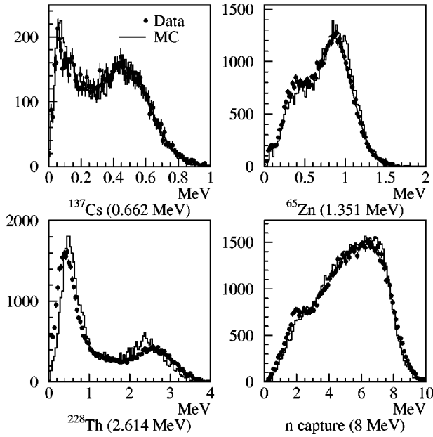
FIG. 7. The total energy reconstructed for various sources compared for data and Monte Carlo simulation.
