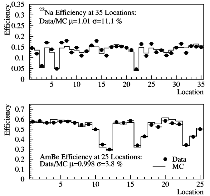
FIG. 11. Comparison of data and Monte Carlo detection efficiency for ^{22}\text{Na} and Am-Be source runs at various locations. Locations at the edges of the detector tend to have lower efficiencies.
