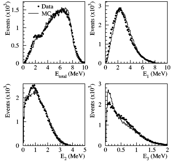
FIG. 13. The Monte Carlo simulation and the data compared for the spectra of total energy and first, second, and third most energetic hit ( E_{\text{total}} , E_1 , E_2 , and E_3 ) digitized in the Am-Be calibration runs.
