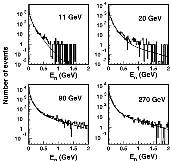
FIG. 4. Energy spectrum of neutrons at different muon energies together with our parametrization. We find \chi^2/N_{\text{DF}} of 3.9, 4.5, 9.6, and 3.7 for 11, 20, 90, and 270 GeV, respectively.
