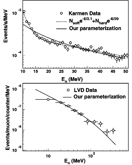
FIG. 5. Comparison of measured neutron energy spectrum with our parametrization.
