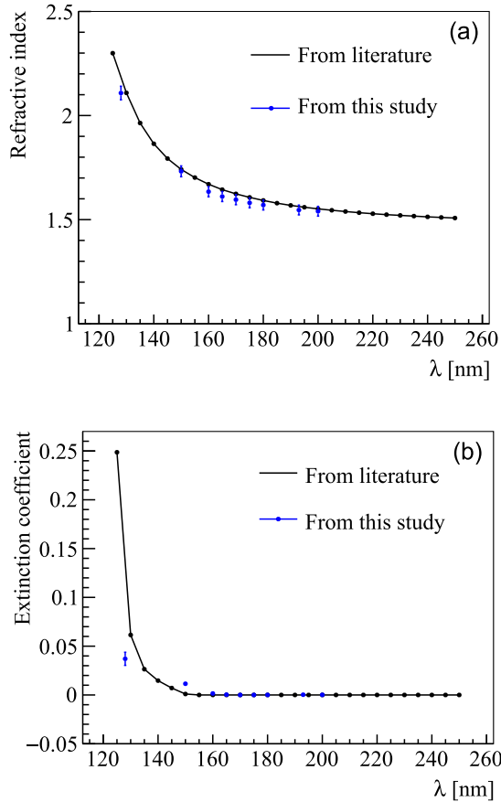
Fig. 8. (a) Fitted refractive index and (b) extinction coefficient of \text{SiO}_2 film, compared to results from the literature [23] (black lines).
