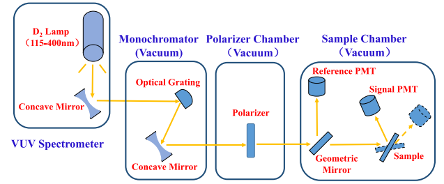
Fig. 1. Schematic of the specular reflection optical system. (From left to right: VUV spectrometer, monochromator chamber, polarization chamber, and sample chamber.)
