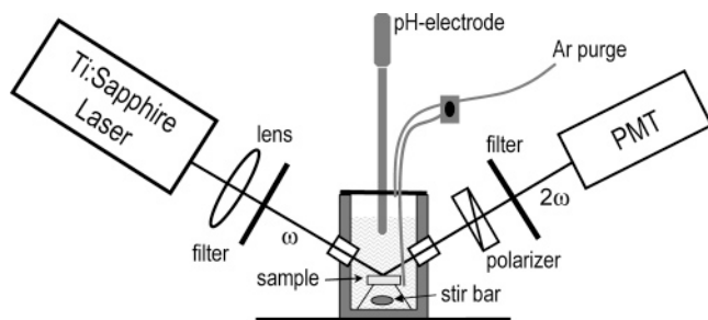
Figure 2. SHG experimental configuration and titration cell.
