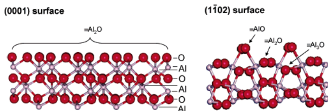
Figure 1. Side views of oxygen-terminated \alpha - \text{Al}_2\text{O}_3 (0001) and ( 1\bar{1}02 ) surfaces that are consistent with hydrated structures proposed based on X-ray reflectivity studies. 13,14 The (0001) surface is terminated by O atoms coordinated to two Al atoms (i.e., \equiv\text{Al}_2\text{O} or doubly coordinated oxygen atoms), while the ( 1\bar{1}02 ) surface is terminated by equal numbers of singly ( \equiv\text{AlO} ), doubly ( \equiv\text{Al}_2\text{O} ) and triply ( \equiv\text{Al}_3\text{O} ) coordinated oxygen atoms. Hydrogen atoms are not shown.
