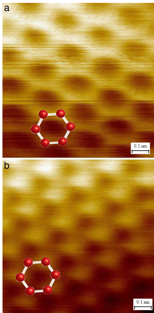
Fig. 2. STM topographic images of different regions of the graphene flake of Fig. 1. The images were obtained with V_{\text{bias}} = +1 V (sample potential), I = 1 nA, and a scan area of 1 nm ^2 . A model of the underlying atomic structure is shown as a guide to the eye. (a) Image from a single layer of graphene (region I of Fig. 1). A honeycomb structure is observed. (b) Image of the multilayer portion of the sample (region II of Fig. 1). The characteristic three-for-six STM image of the surface of bulk graphite is observed.
