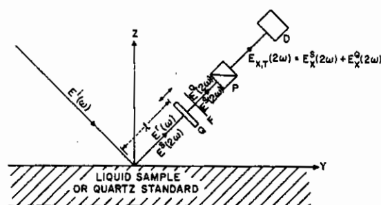
Fig. 1. Experimental scheme for phase measurements. Q, reference quartz; P, analyzer; D, monochromator and detector assembly. E^i and E^r are respectively, the incident and reflected fundamental field amplitudes; E^S and E^Q , the SH fields generated by the sample (or quartz standard) and the reference quartz, respectively; E_x^S , E_x^Q and E_{x,T} , the x components of the SH field due to the sample, reference, and their sum, respectively.
