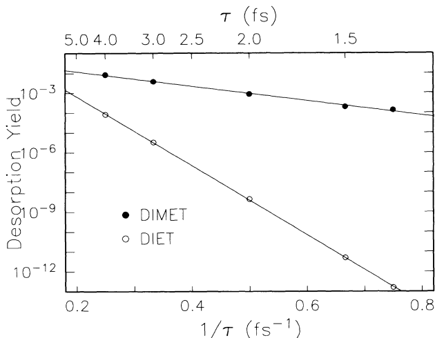
FIG. 3. Desorption probability by DIMET ( P_{\text{DIMET}} ) and by single-excitation DIET ( P_1 ) as a function of excited-state lifetime \tau obtained from trajectory calculations with a peak electronic temperature of 5500 K.
