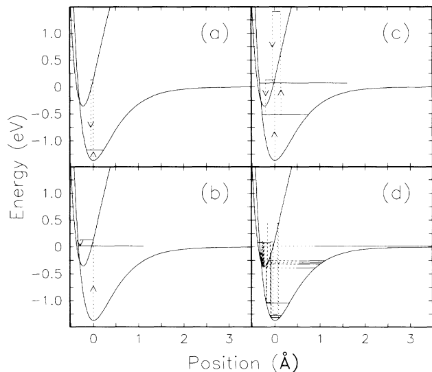
FIG. 1. Trajectories for motion on the ground and excited PES. The dotted lines represent the total energy of the adsorbate complex, with vertical segments arising from Franck-Condon transitions and horizontal segments from conservative motion on a given PES. (a),(b) Trajectories displayed associated with a single-excitation DIET process. (a) and (b) correspond, respectively, to cases where the particle remains in the excited PES for less than or greater than \tau_c , the critical time for desorption. (c),(d) Trajectories for the DIMET process. (c) is a simplified example of DIMET with two excitation-deexcitation cycles, while (d) is the result of a complete simulation with \tau = 2 fs and peak electronic temperature of T_e = 5500 K.
