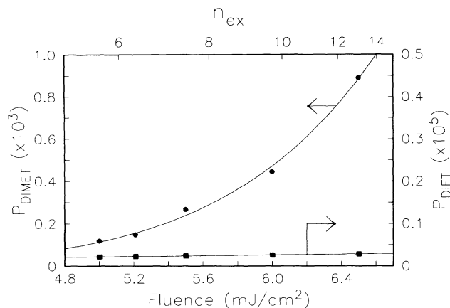
FIG. 2. Desorption probability for DIMET and an upper bound for a DIET as a function of laser fluence from stochastic trajectory simulations (shown together with power-law fits). The corresponding average number of excitations for all adsorbates in the DIMET calculation is indicated in the upper scale. The range of fluences corresponds to peak T_e between 4600 and 5500 K. The excited-state lifetime is \tau = 2 fs.
