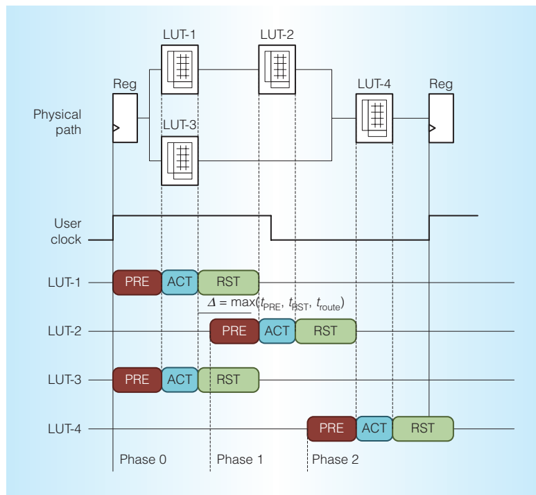
Figure 2. The timing diagram and critical path for a chain of four DRAF lookup tables. Each clock cycle is decomposed into three phases. LUT-1 and LUT-3 are in phase 0, LUT-2 is in phase 1, and LUT-4 is in phase 2. \Delta represents the three-way overlapping of restoration, precharging, and routing delays.
