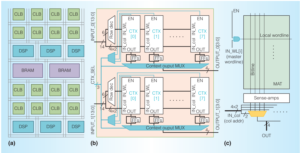
Figure 1. The DRAM-Based Reconfigurable Acceleration Fabric (DRAF) architecture. (a) The block layout of DRAF, similar to an FPGA. Block sizes and numbers can vary across devices. (b) The configurable logic block (CLB) in DRAF. As a typical example, a CLB contains two DRAM-based lookup tables and associated flip-flops (FFs) organized into eight contexts. Each lookup table has an 8-bit (6 bits for row and 2 bits for column) input and a 4-bit output. (c) Detailed view of one context in a DRAF lookup table with the context enable gate and specialized column logic.
