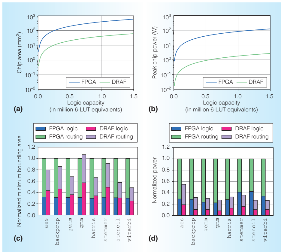
Figure 3. Area and power comparison between DRAF and a conventional FPGA. (a, b) Device-level comparison. (c, d) Comparison after real application mapping.
