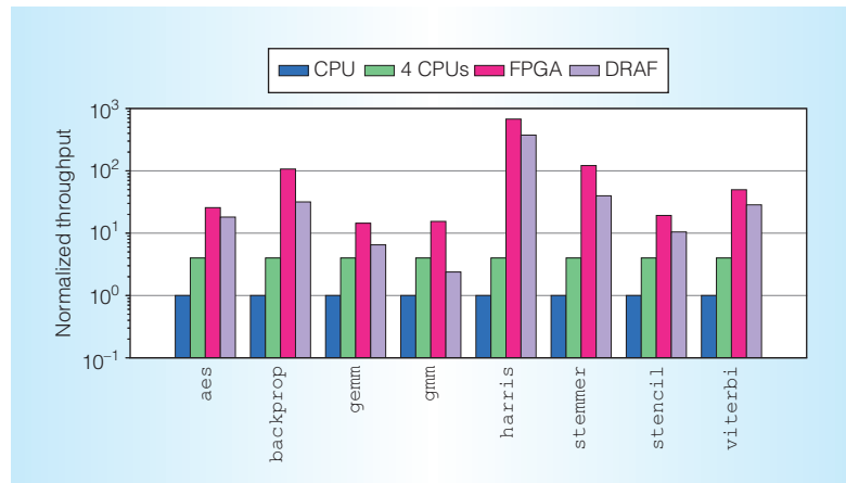
Figure 4. Performance comparison between single-core, multicore, FPGA, and DRAF using representative datacenter application kernels. Assume ideal scaling from single-core to multicore platform.
