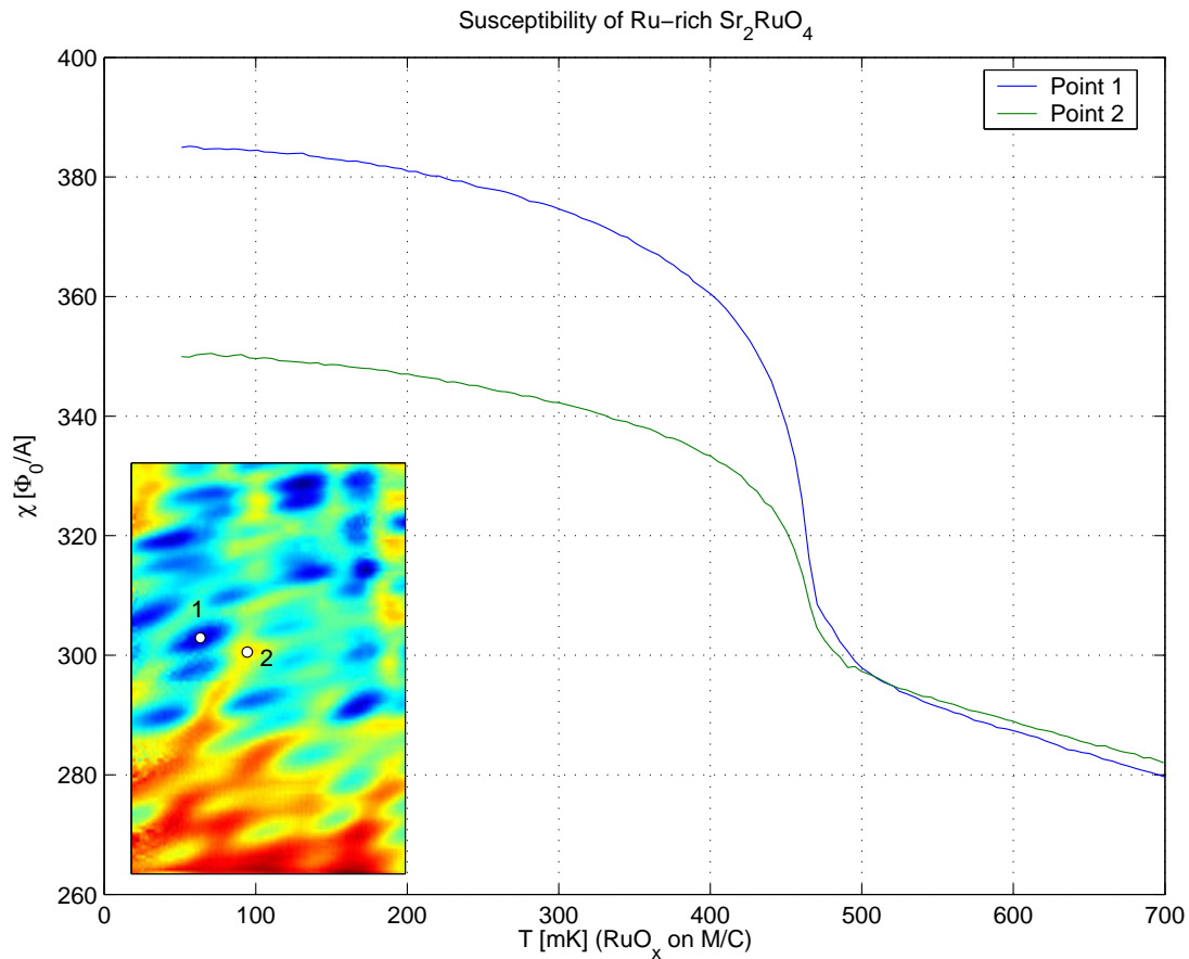
Figure 7.3: Temperature dependence of the local susceptibility of a 3K phase. The blue curve corresponds to a point with strong additional susceptibility response below 0.45 K (Point 1 in the inset figure), while the green curve is the response at a nearby low-response point (Point 2). Inset: Scan of the sample at 100 mK, where the Ru inclusions show up as areas with strong susceptibility response.
