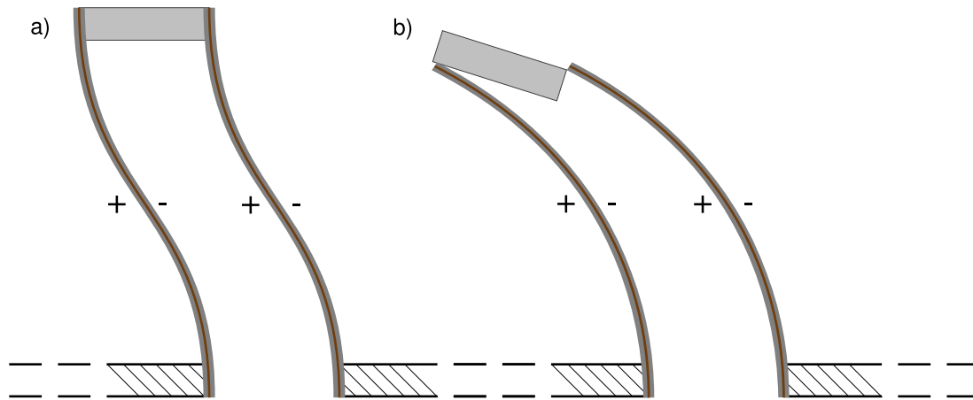
Figure 2.3: The bimorphs used bend in an S shape in order to allow for parallel uniaxial motion of the scan head relative to the base. a) Illustration of the scan stage movement (the range of motion is greatly exaggerated for clarity). (b) Ordinary “cantilever” bimorphs are not suitable for this type of scanner, since they would not allow a square connection with two parallel benders to move.
