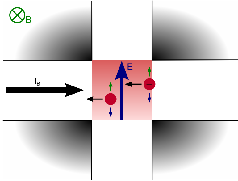
Figure 4.1: A Hall sensor in a magnetic field \vec{B} . The Lorentz force caused by the motion of the charge carriers in a B field is balanced by the force from the E field originating in the charge gradient across the sensor.
