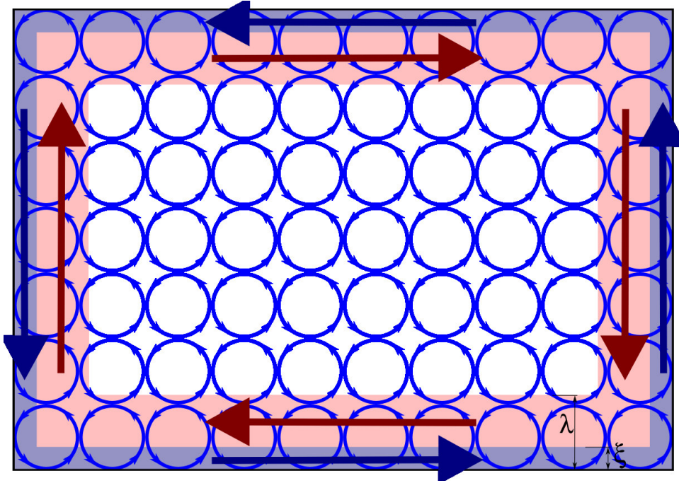
Figure 6.1: A cartoon for explaining the current flows and magnetic fields associated with TRSB in a superconductor with all electrons paired in L=1 Cooper pairs. Modeling the pairs as orbiting electrons, in the interior there is no net current since neighboring electron pairs cancel out; however, at an edge this cancellation is broken and there is a current within a distance \xi from the surface, flowing as indicated by the blue arrows. The magnetic field generated by this current is canceled by a counterflowing current on the length scale of \lambda because of the Meissner effect.
