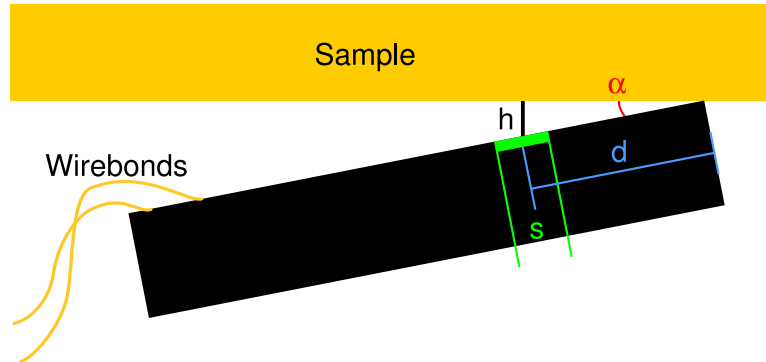
Figure 2.1: The sensor in a scanning chip-sensor microscope is aligned at a shallow angle with respect to the sample in order to minimize the sensor height. The spatial resolution of the microscope is determined by both the sensor active area size ( s ) and the height ( h ). Since wirebonds can be the limiting factor for the probe angle, it is important that the probe is designed with the wirebonds as far back as possible on the probe chip.
