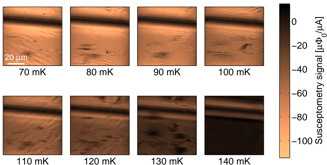
Figure 5.5: Susceptibility images the TES film. The small-length-scale variations in the susceptibility may be caused by the SQUID occasionally touching and locally heating the sample and may thus not be actual variations in the sample.
