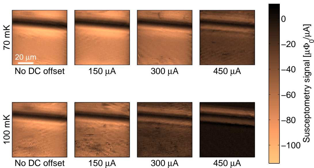
Figure 5.6: Susceptometry images with a background field applied using the field coils. The applied AC current for the susceptometry is 50\mu\text{A} . The DC offset current through the field coil is indicated on each scan.
