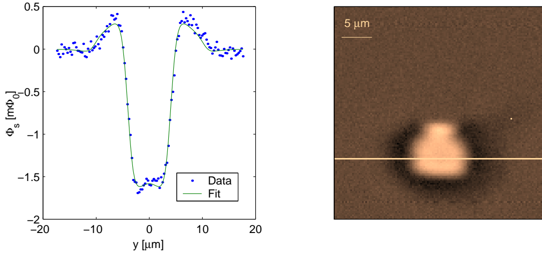
Figure 5.2: (a) Best fit of calculated SQUID response to data for a 3\mu\text{m} tin disk at 30mK, height= 1.9\mu\text{m} . (b) The corresponding full image, with the cross section marked with a bright line.
