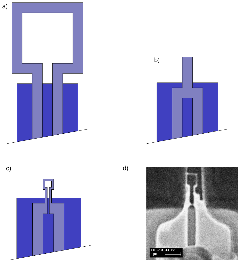
Figure 3.5: Attempts to modify specially designed 1st-generation SQUIDs using e-beam lithography in order to produce submicron pickup loops. a) The regular 1st-generation SQUIDs have pickup loops fabricated using the HYPRES photolithographic process. Lithography limits set a practical lower bound on the pickup loop size of 8 \mu\text{m} . b) The pickup loop was replaced by a tab in order to make e-beam lithography modifications possible. c) Sketch of one attempted pickup loop geometry. d) Electron micrograph of one of the attempts to fabricate the geometry in (c) that was closest to succeeding.
