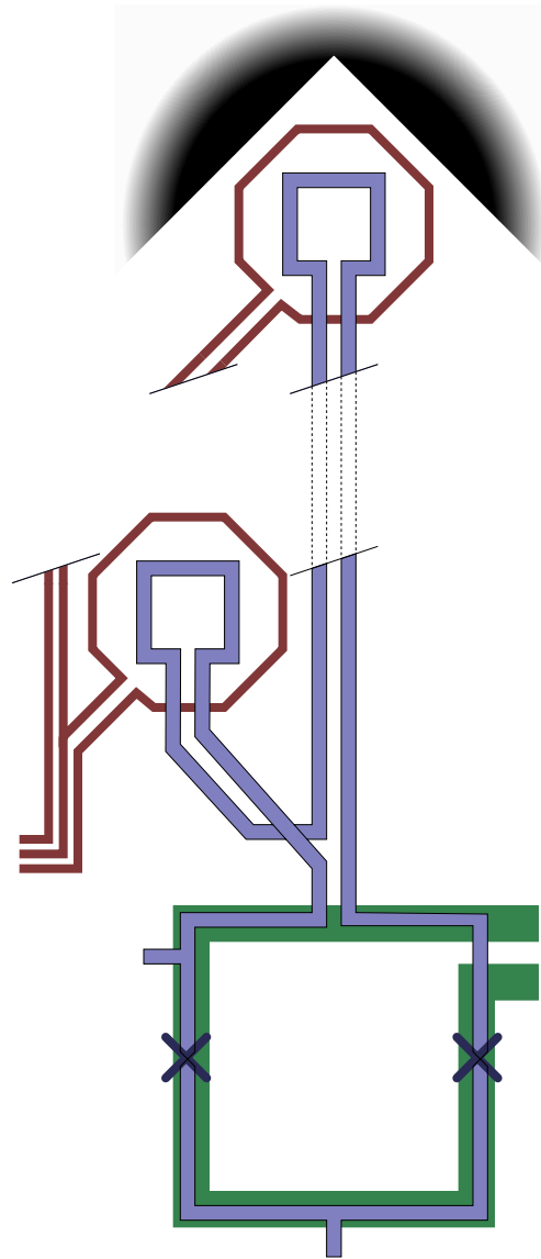
Figure 3.3: a) A sketch of the design of our “first-generation” scanning SQUID design. b) Micrograph of the square front SQUID pickup loop, with a tip polished to a distance of around 30 \mu\text{m} from the center of the pickup loop. The polishing distance is limited by the octagonal field coil.
