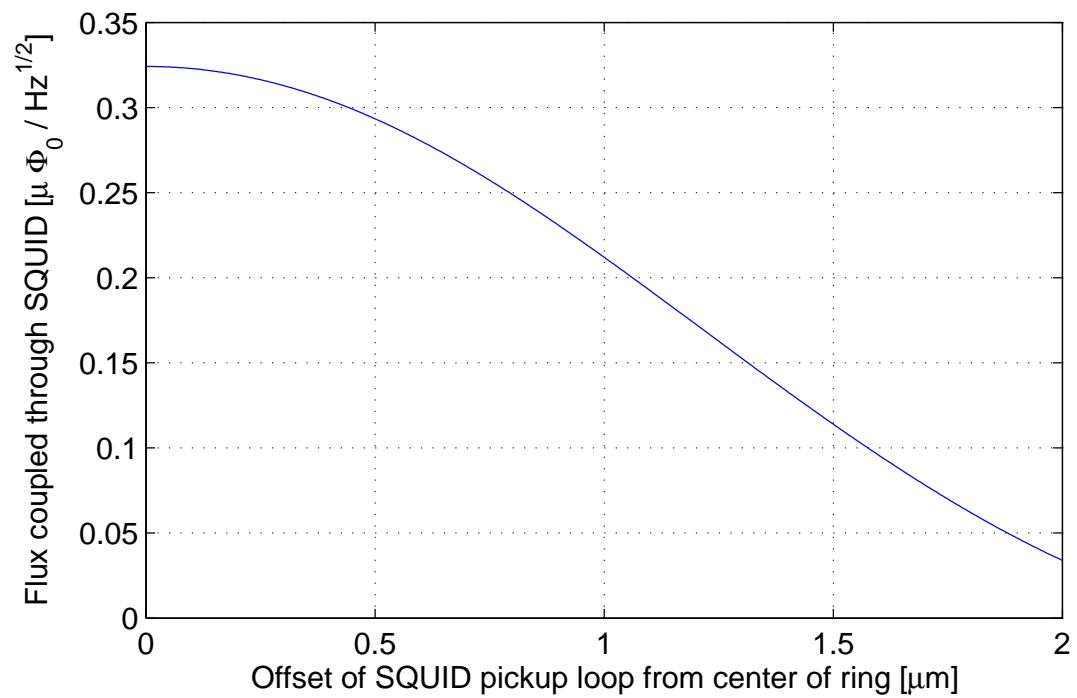
Figure 3.10: Calculated magnetic coupling of ring of diameter 2 \mu\text{m} to a 4 \mu\text{m} diameter SQUID pickup loop 1 \mu\text{m} above the ring, as a function of the offset of the ring center from the center of the pickup loop.
