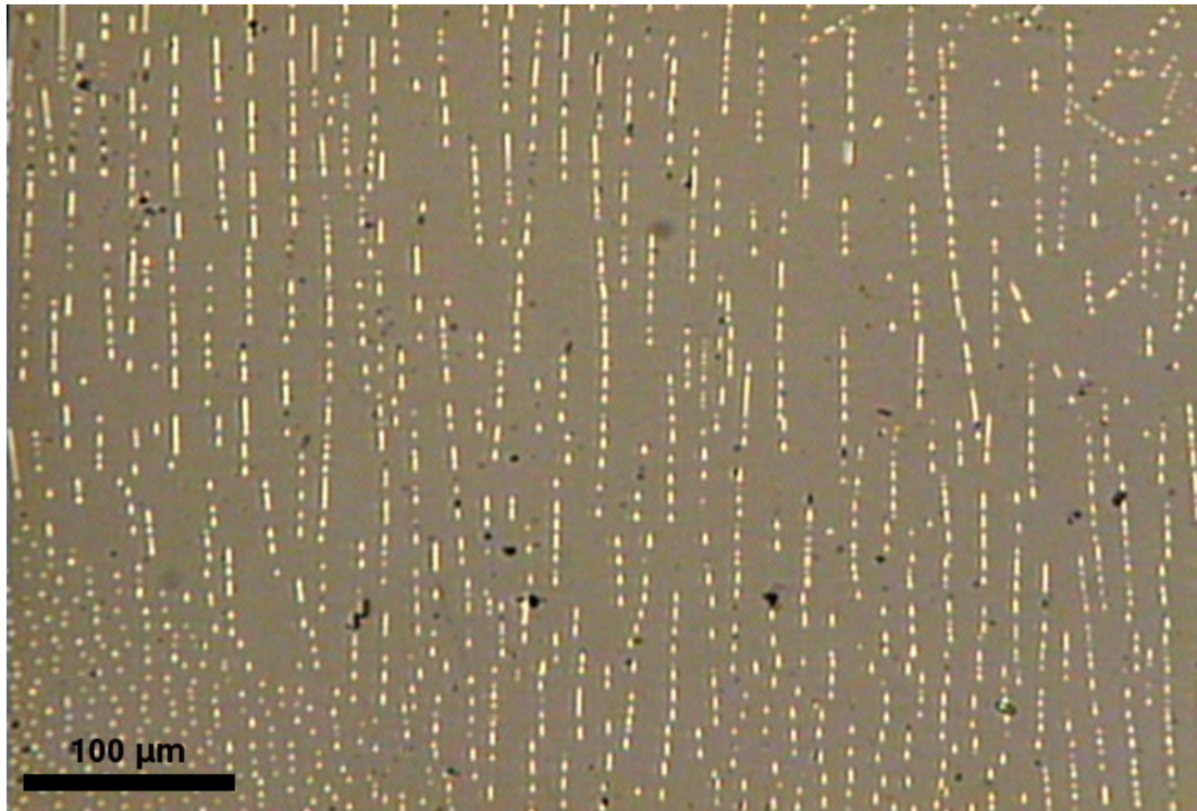
Figure 7.1: Micrograph of the 3K phase sample studied. The Ru inclusions in the sample are visible as bright spots. The inclusions are distributed unevenly in the sample. We attempted to scan an area where the inclusions could be seen individually with our scanning SQUID resolution.
