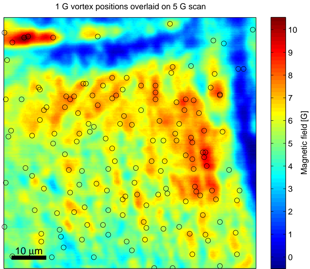
Figure 6.8: Overlay of the vortex positions in the 1 G scan on the 5 G scan data; the data is the same as in Fig. 6.7. The vortex positions in the 1 G scan are marked with circles. The vortices tend to line up in the same areas even though the sample has been thermal cycled above T_C between the measurements.
