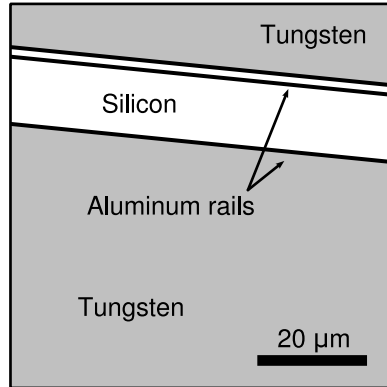
Figure 5.3: Sketch of the part of the W transition edge sensor visible in the scans.
