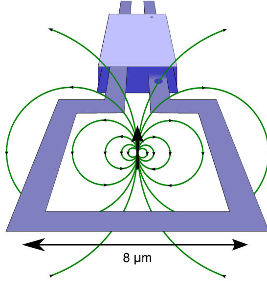
Figure 5.1: A dipole in the 8 \mu\text{m} pickup loop of one of our Generation 1 SQUIDS. The flux from the dipole through the SQUID must typically be calculated numerically when comparing measurement results to theoretical models.
