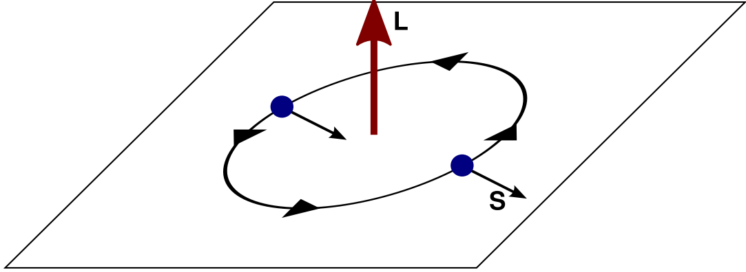
Figure 6.2: A real-space visualization of a k_x + ik_y class order parameter. The blue dots are electrons. S indicates the electron spin and L indicates the orbital angular momentum of the Cooper pair.
