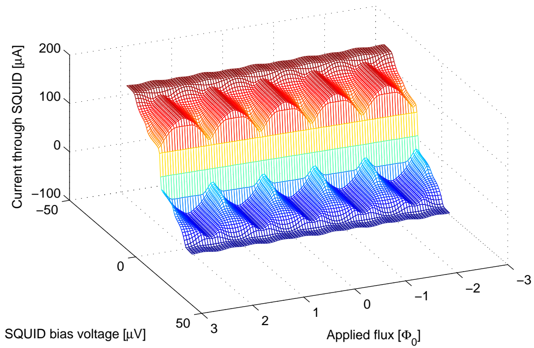
Figure 3.7: Measured flux-voltage-current landscape for a second-generation SQUID at 4K.
