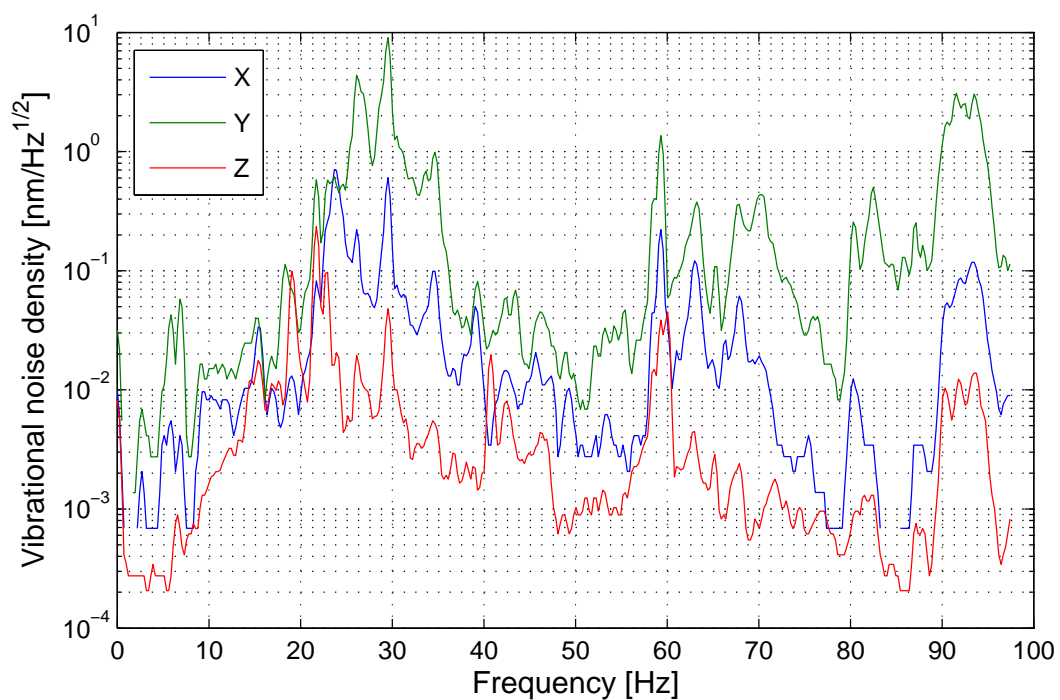
Figure 2.7: Vibration spectra measured at room temperature by connecting the piezo driver lines to a spectrum analyzer. The Y piezo has larger vibrations than the others, presumably because the driven mass includes the mass of the X piezo bender pair.
