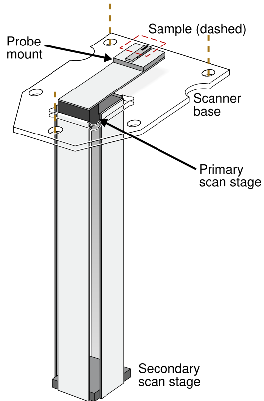
Figure 2.4: Sketch of the scanner. One pair of 2" long S -bender piezoelectric bimorphs connect the scanner base to the secondary scan stage and provide motion in the Y direction; a second pair connect the secondary and primary scan stages provide the X axis motion. A standard 1" cantilever bimorph provides the Z axis motion; the probe mount is attached at the end of this bimorph. The scanner is mounted using three spring-loaded screws to a copper baseplate.
