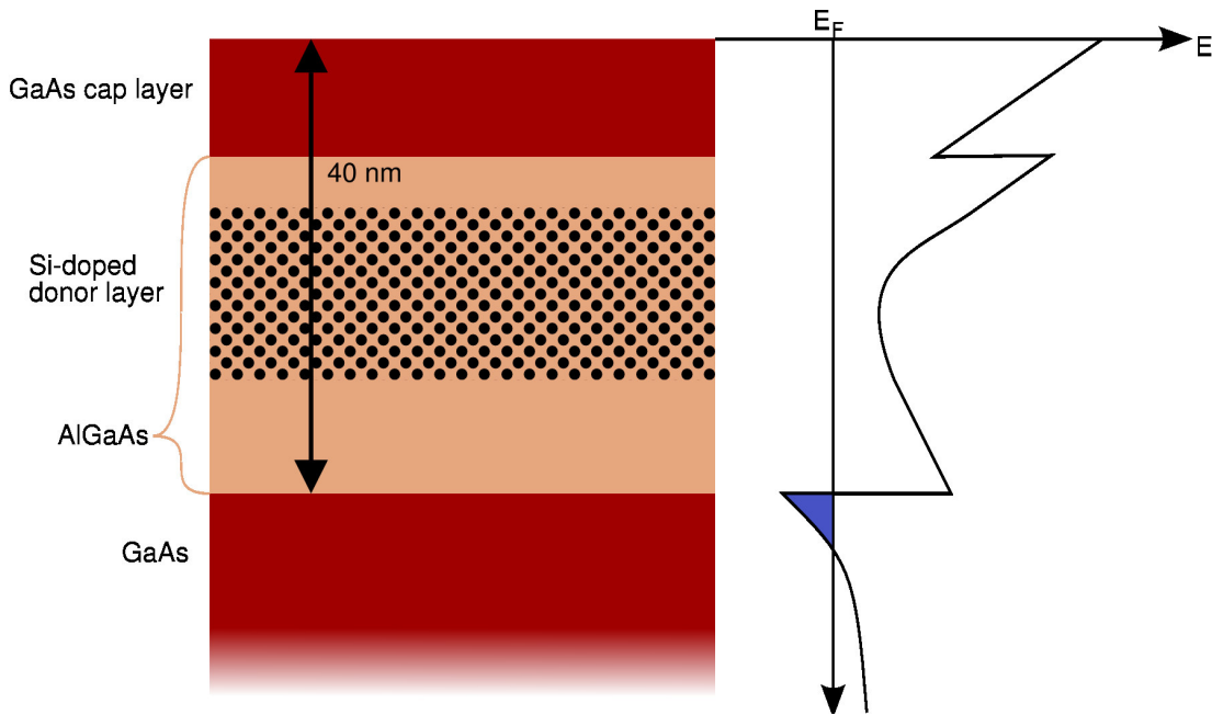
Figure 4.2: Illustration of the 2DEG structure used for the generation 3 and 4 Hall probes. The energy level diagram, based on calculations by C. W. Hicks, is shown on the right-hand side. The 2DEG forms at the GaAs/AlGaAs interface.
