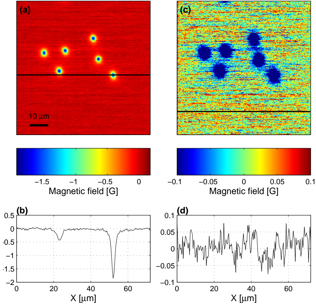
Figure 6.6: Scanning Hall probe image of the sample shown in figure 6.3, cooled in a background field of \sim 25 mG. The background has been line normalized to remove 1/f noise. (a) Image with a color scale showing the full measured magnetic field range. Isolated trapped vortices dominate the image. (b) Cross section taken along the black line in (a). (c) Image with an expanded color scale, showing that there are no obvious features in the noise. (d) Cross section taken along the black line in (c).
