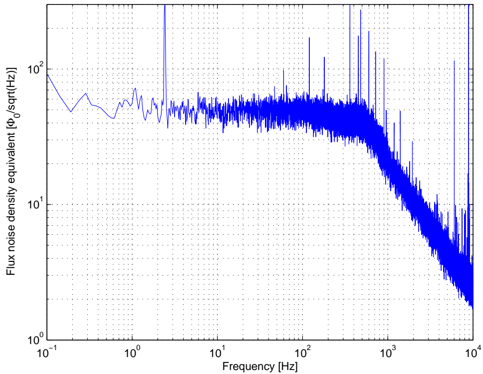
Figure 3.4: Typical noise of the first-generation scanning SQUIDs in an AC feedback loop, with a white noise level around 50 \mu\Phi_0/\sqrt{\text{Hz}} . The knee around 500 Hz is due to bandwidth limitations in the system. This noise is significantly higher than the intrinsic noise of the SQUIDs as measured directly in a setup without the feedback loop.
