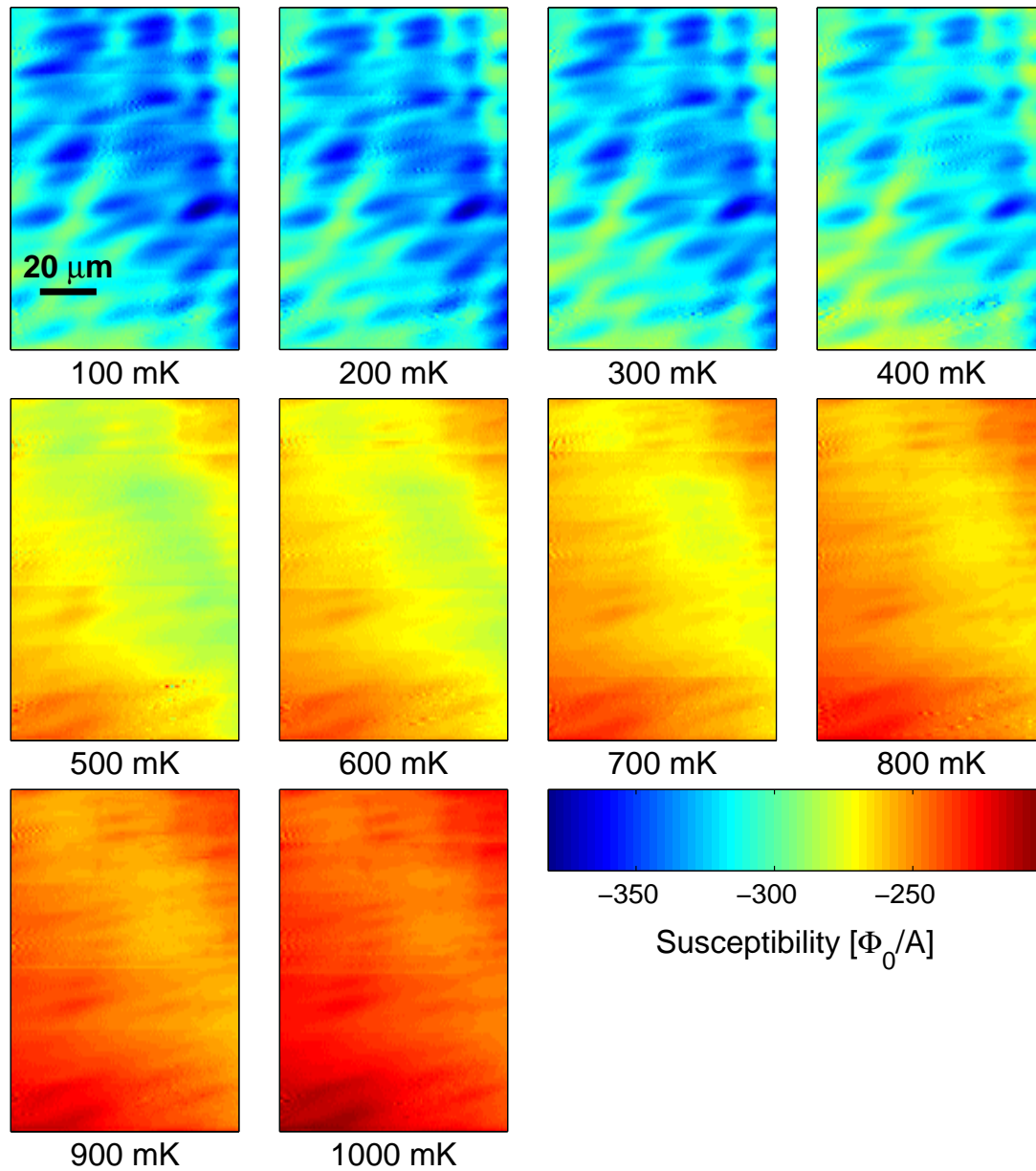
Figure 7.2: Scans of the 3K phase sample at temperatures up to 1K. The susceptibility is relatively uniform above the bulk Ru T_c , but becomes strikingly inhomogeneous below that temperature.
