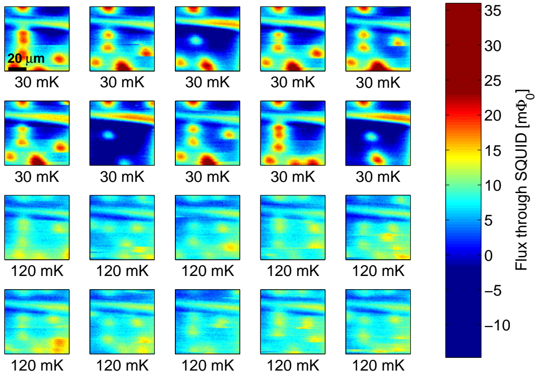
Figure 5.4: Sequential magnetometry images of the TES sensor at 30 and 120 mK. The vortices are significantly more well-defined at 30 mK, indicating that \lambda is (as expected) much smaller at that temperature, but at both temperatures the pinning appears to be relatively weak since there are large changes between consecutive images. The sudden jumps in the figures are vortices moving during the scan.
