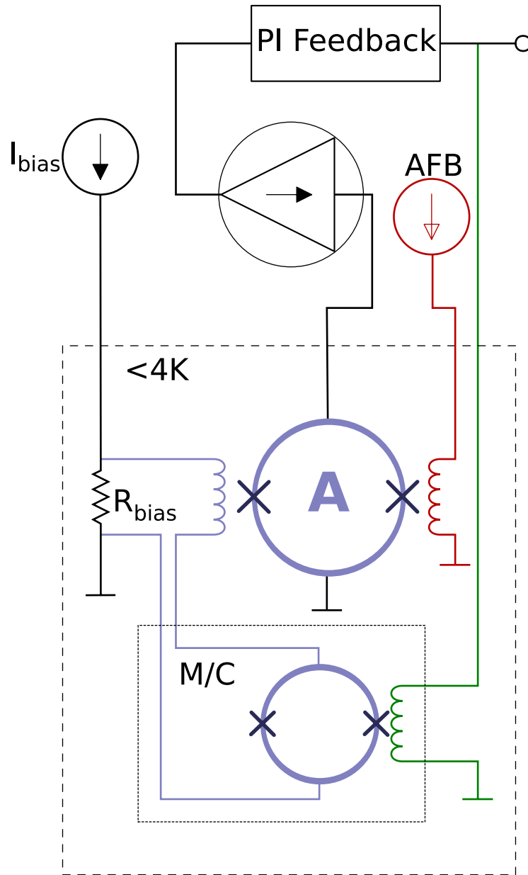
Figure 3.8: The DC feedback loop with a SQUID array used as a low-temperature preamplifier. The susceptometer SQUID (at the bottom) is voltage biased using a small resistor. A SQUID array is used to measure the current through the susceptometer. Linearization is achieved by feeding back flux into the susceptometer, while the array is DC flux biased at a suitable operating point.
