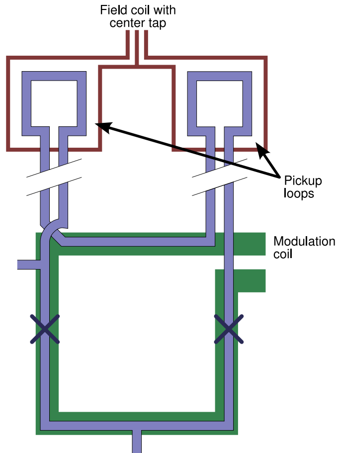
Figure 3.2: Sketch illustrating the fundamentals of Ketchen's SQUID susceptometer. The two pickup counterwound pickup loops with surrounding field coils allow a magnetic field to be applied locally, only measuring the magnetic response of a sample placed in one of the pickup loops.
