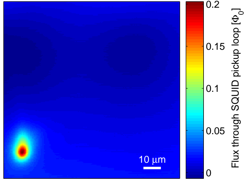
Figure 6.4: Scanning SQUID image of a single crystal of \text{Sr}_2\text{RuO}_4 with a single vortex within the field of view. The only other magnetic signals visible are a smoothly varying background.
