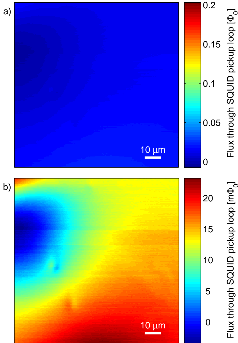
Figure 6.5: Scanning SQUID image of the same area of a \text{Sr}_2\text{RuO}_4 crystal as in Fig. 6.4 but with the background field compensated so that there are no vortices. In (a), the color scale is the same as for Fig. 6.4, while (b) is the same image with the color scale stretched to enhance detail. The only visible features apart from the smooth background (which may be caused by the secondary pickup loop hanging off the sample) are dipole-like structures that are visible both in the superconducting and normal state (measured at 4 K) and thus appear to be magnetic particles stuck on the surface.
