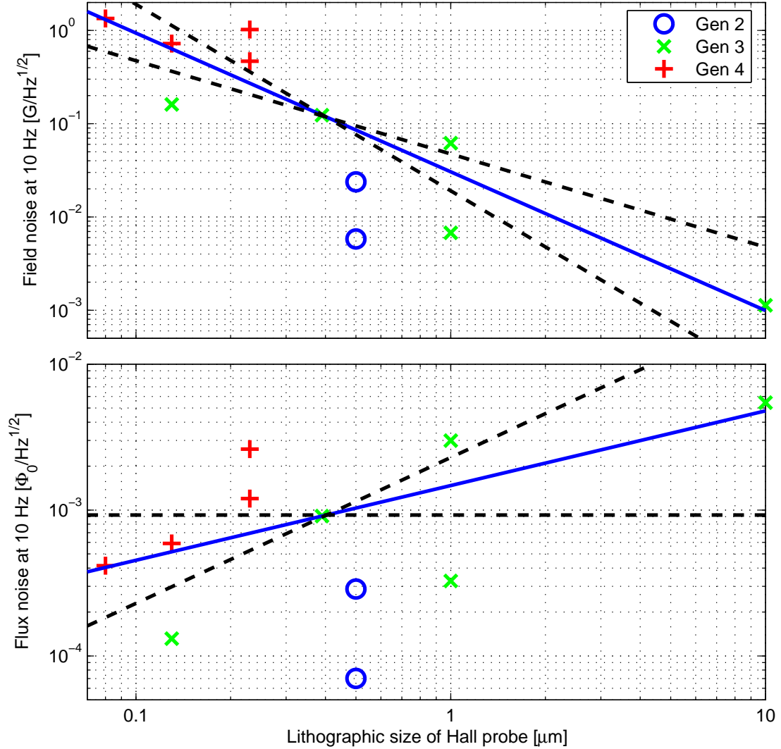
Figure 4.5: Noise level at 10 Hz for Hall probes used in the Moler lab, at the measured optimal current for each probe. Generations are explained in Table 4.1. The noise roughly appears to follow a power law. The fit is calculated using only the data for the Gen. 3 and 4 Hall probes, since the Gen. 2 probes were fabricated on a different 2DEG. The best fit for the field noise is 0.0305 \times s^{-1.48} ; fits with the exponent forced to -1 and -2 are represented by the dashed lines.
