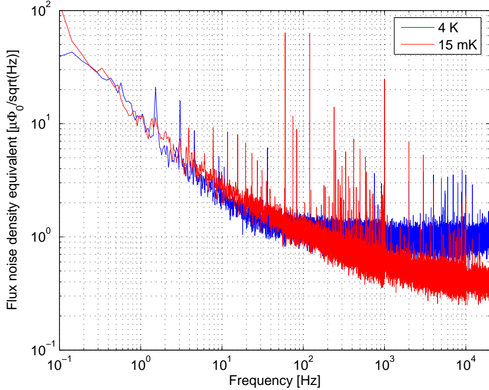
Figure 3.9: Comparison of the SQUID noise at 4 K and at the dilution refrigerator mixing chamber temperature of 15 mK.
