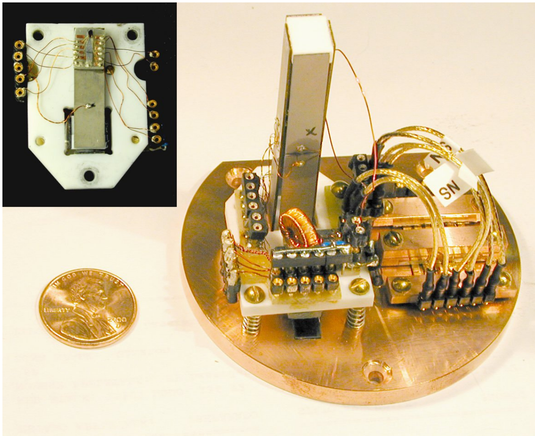
Figure 2.2: Photo of the scanning microscope mounted on the copper baseplate. The sample is mounted directly on the baseplate. Wiring is heatsunk either using the sapphire stripline heatsink on the right-hand-side of the baseplate, or by wrapping around copper bobbins such as the one visible in the back of the figure. Inset: Bottom view of the scanner with the probe mount mounted on the Z axis bender.
