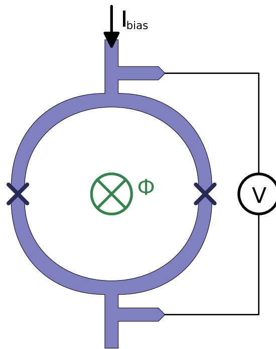
Figure 3.1: A DC SQUID is basically a superconducting loop with two Josephson junctions. At a given bias current (above the junction critical current) the voltage across the SQUID is periodic in the flux threading the loop.
