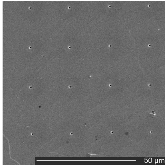
Figure 6.3: An SEM image of the \text{Sr}_2\text{RuO}_4 crystal used for the Hall probe imaging. An array of holes was milled in the sample using a FIB. The hole spacing is 20 \mu\text{m} .
