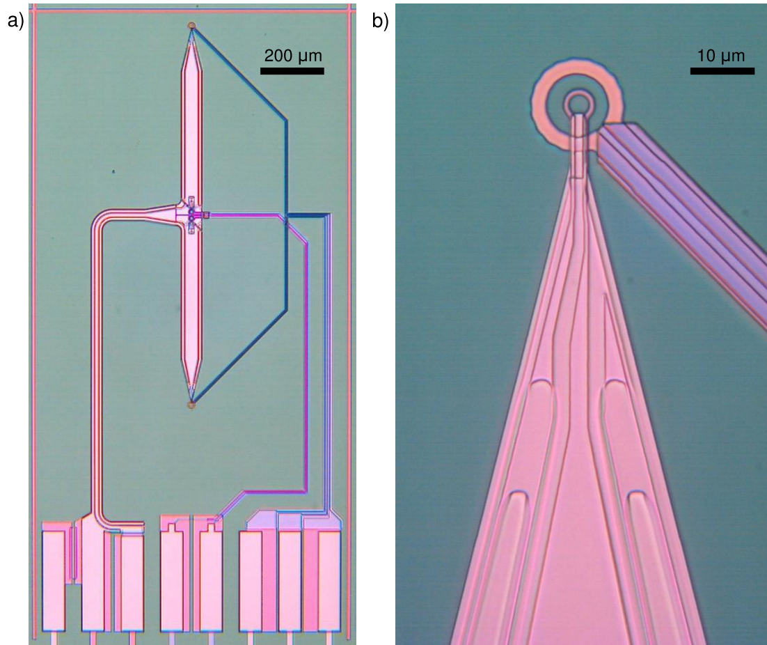
Figure 3.6: The 2 nd generation scanning SQUID design. (a) A full SQUID chip with a 4 μm pickup loop. (b) Close-up of the pickup loop area.
