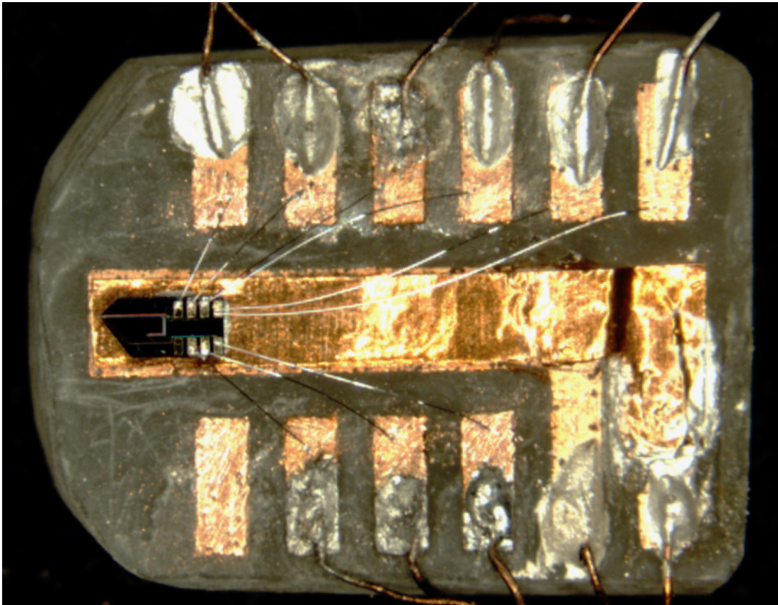
Figure 2.5: Photo of a mount with a SQUID; similar mounts are used for Hall probes.
