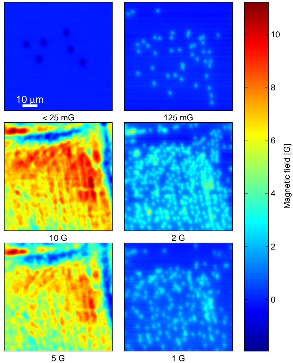
Figure 6.7: Hall probe scans in varying magnetic fields. The vortices appear to form lines that are spaced much more closely than the FIB-milled hole pattern. There are also regions at the top and right-hand side of the imaged area in which the density of vortices is much lower than the average in the images.
