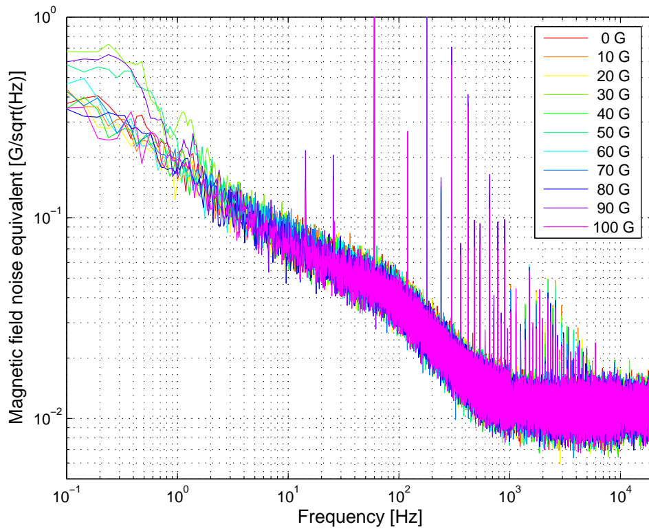
Figure 4.4: Comparison of noise measurements on a 0.39 \mu\text{m} Hall probe at 15 mK with a range of applied fields. There is no significant difference between the noise levels at different applied fields; the small difference seen at very low frequencies, which appears to vary randomly with the applied field, is likely due to a random variation in the number of discrete switching events.
