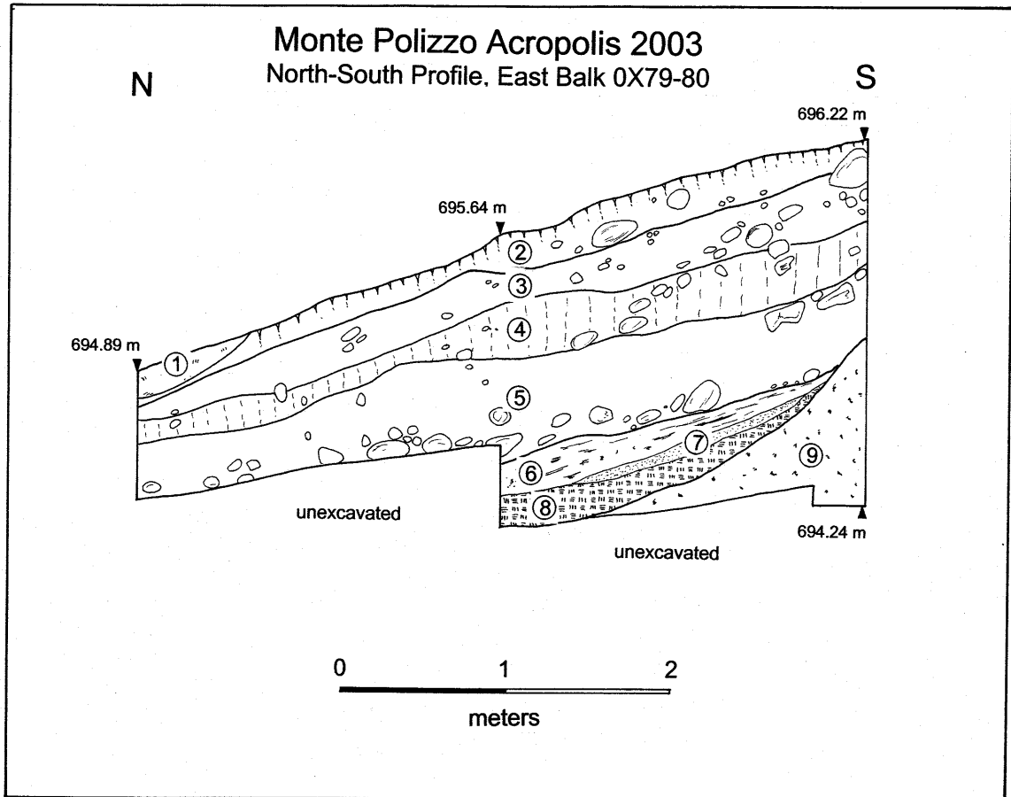
Fig. 3.17 Profile drawing, west balk of trench 0X79-80, zone E, 2003
