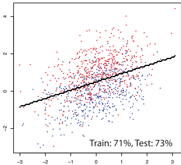
Linear Discriminant Analysis
