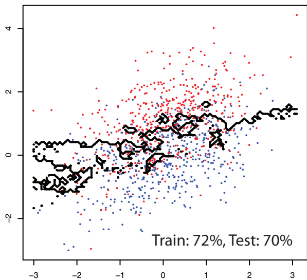
K-Nearest-Neighbor (k=20)
