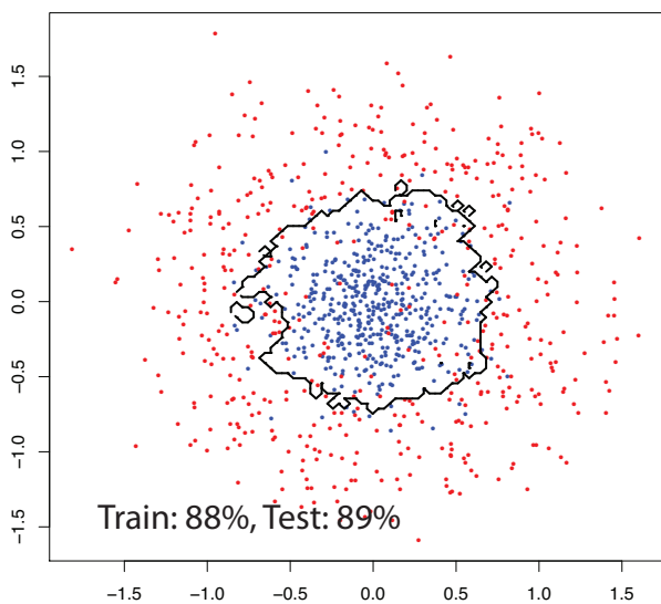
K-Nearest-Neighbor (k=20)
