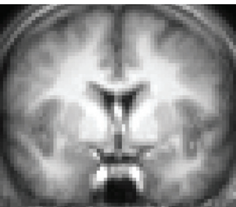
SPM nonlinear (100)
