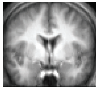
SPM nonlinear (100)
