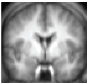
SPM nonlinear (12)
