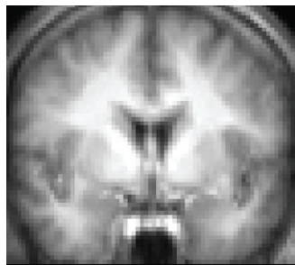
SPM DARTEL
