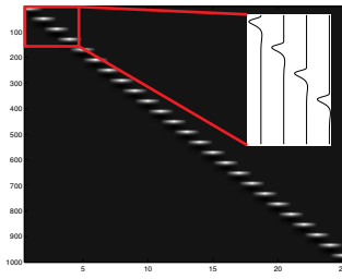
Beta series design matrix
