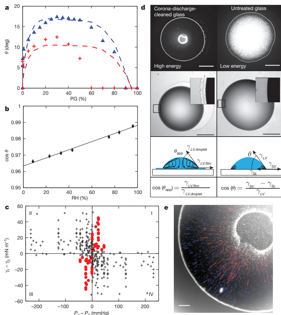
Figure 2 | Individual droplet characteristics.
