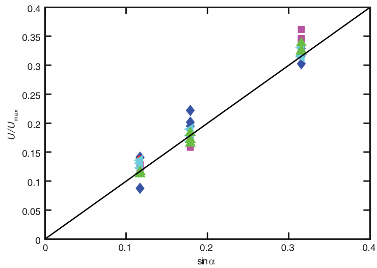
Extended Data Figure 8 | U/U_{\max} as a function of \sin \alpha . Shown for the cutoff constant, l_n = 11.2 , for 10% PG droplets of 0.25 µl (blue), 0.5 µl (red), 0.75 µl (magenta), 1 µl (cyan), 1.5 µl (green). The solid line represents the
