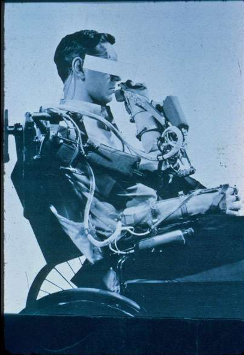
Reswick advertisement BME - Case REO arm aid Mark I - 08/1974
