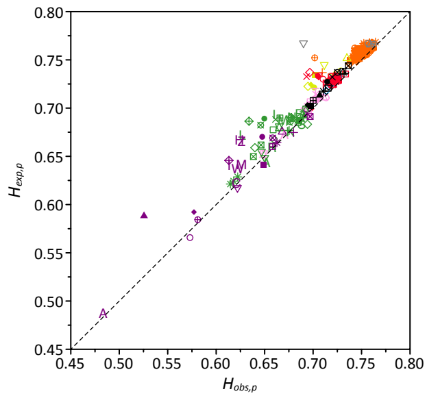
Figure S2. Expected versus observed heterozygosity across populations ( r=0.975 , P<10^{-16} ). Populations are indicated by the same symbols as in Figure 3 . The black dashed line depicts the identity line.
