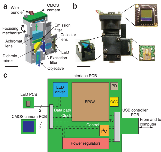
Figure 1 | Design and fabrication of an integrated fluorescence microscope. (a) Computer-assisted design of an integrated microscope, shown in cross-section. Blue and green arrows mark illumination and emission pathways, respectively. (b) Image of an assembled integrated microscope. Insets, filter cube holding dichroic mirror and excitation and emission filters (bottom left), PCB holding the CMOS camera chip (top right) and PCB holding the LED illumination source (bottom right). The wire bundles for LED and CMOS boards are visible. Scale bars, 5 mm (a,b) . (c) Schematic of electronics for real-time image acquisition and control. The LED and CMOS sensor each have their own PCB. These boards are connected to a custom, external PCB via nine fine wires (two to the LED and seven to the camera) encased in a single polyvinyl chloride sheath. The external PCB interfaces with a computer via a USB (universal serial bus) adaptor board. PD, flash programming device; OSC, quartz crystal oscillator; I 2 C, two-wire interintegrated circuit serial communication interface; and FPGA, field-programmable gate array.
