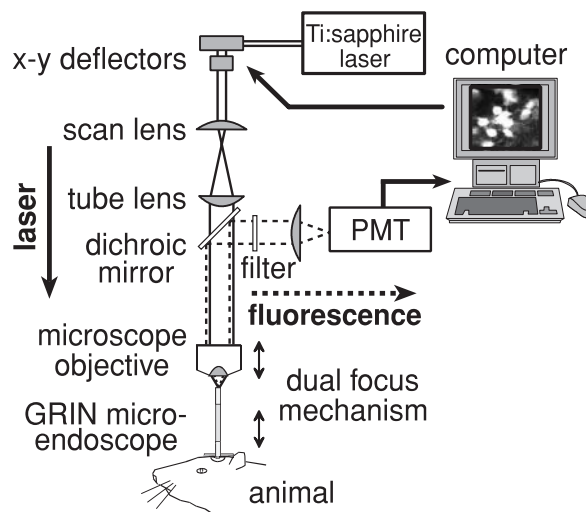
FIG. 7. Optical schematic of the two-photon endoscope. A Ti:sapphire laser emits \sim 100 -fs pulses of infrared excitation light. The laser beam is steered in two angular dimensions by a pair of galvanometer-driven deflector mirrors and is expanded in a telescope comprised of a scan lens and a tube lens. Either a microscope objective or an achromat (not depicted) focuses the beam to a focal spot just above the external face of the endoscope probe. The probe refocuses the lateral scan pattern within the specimen. The focal plane in the specimen may be adjusted by moving either the endoscope probe itself or the microscope objective. This enables one to set the endoscope probe position and to acquire optical sections by adjusting only the position of the microscope objective. Fluorescence emissions (dashed lines) returning from the sample are separated from the excitation beam by a dichroic mirror and detected by a photomultiplier tube (PMT). A computer controls the galvanometer deflectors and reconstructs the image of the sample.
