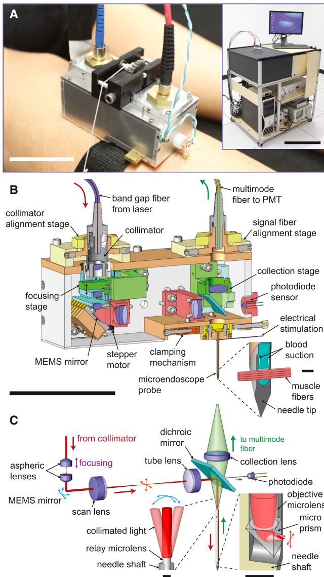
Figure 1. The Wearable Microscope Straps to the Human Body for Imaging Electrically Evoked Motor Unit Twitches
