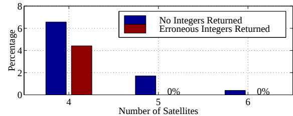
Figure 10 Integer Search Reliability
