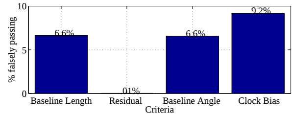
Figure 9 Incorrect integer combinations falsely satisfying criteria for all three baselines
