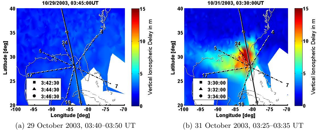
Figure 6.4: SAC-C satellite ground track and ground network measurements of TEC. Black broken line segments point in the direction of the GPS satellites (PRN numbers shown).
