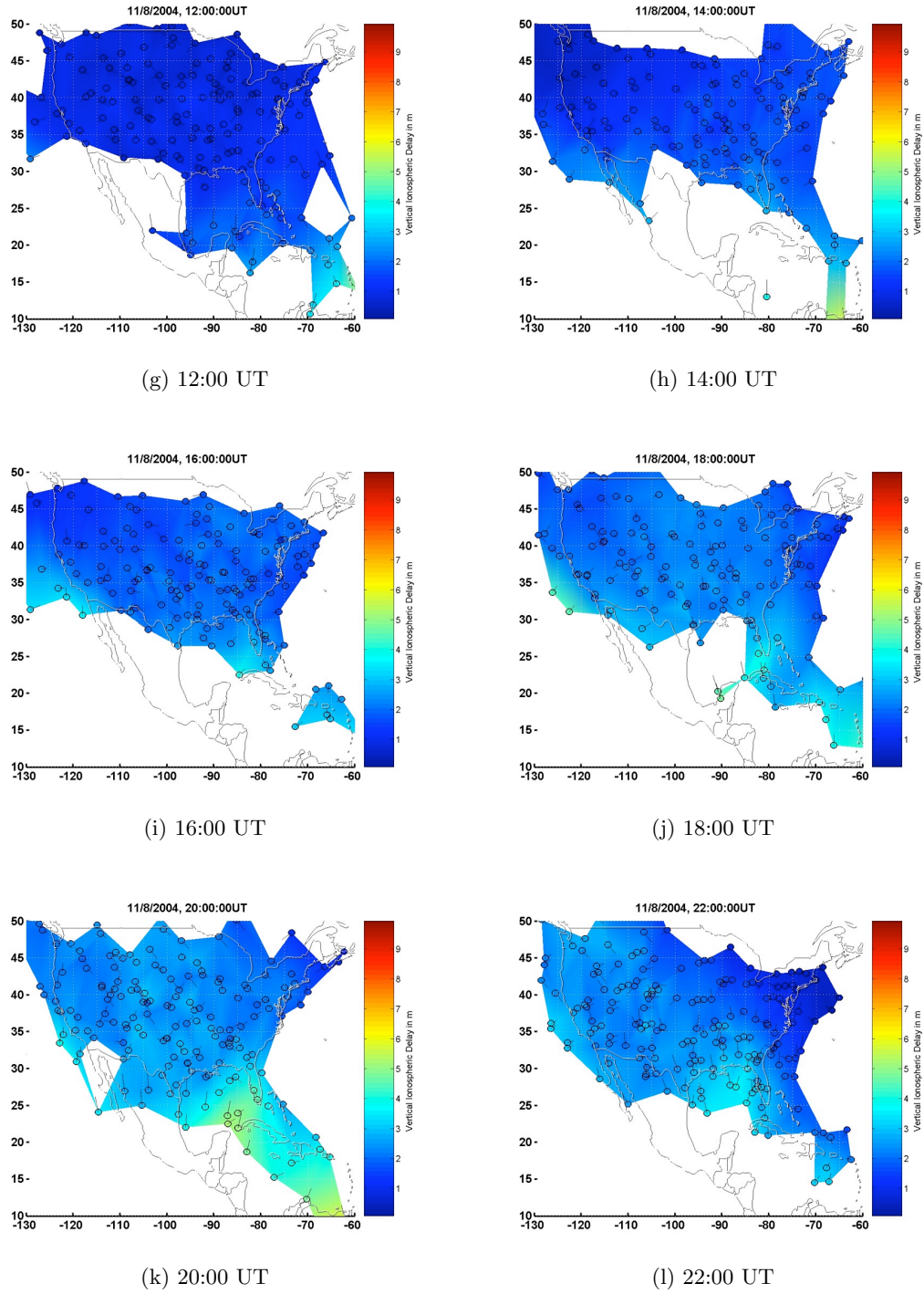
Figure B.13: 8 November 2004, 12:00–22:00 UT.
