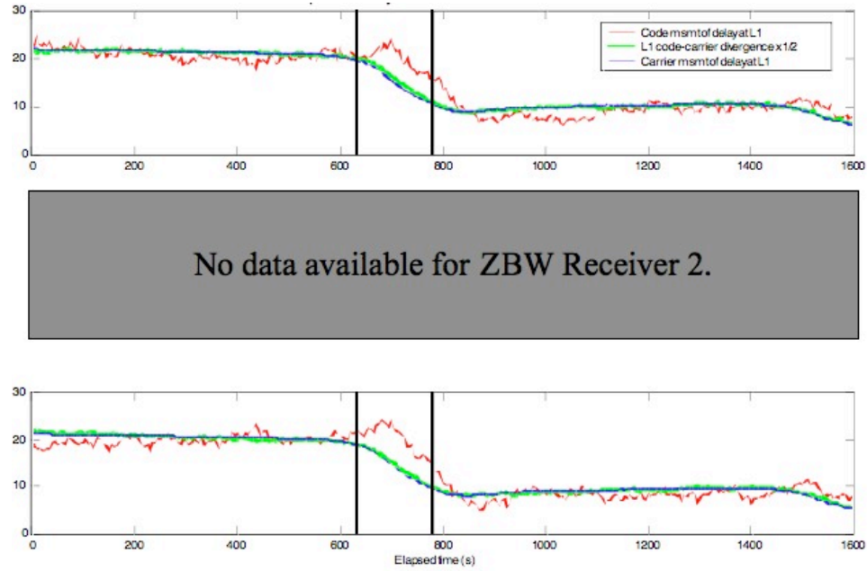
Figure 5.7: Slant ionospheric delay to SVN 24 from each receiver at Boston WAAS station. Data for Receiver 2 not available.
