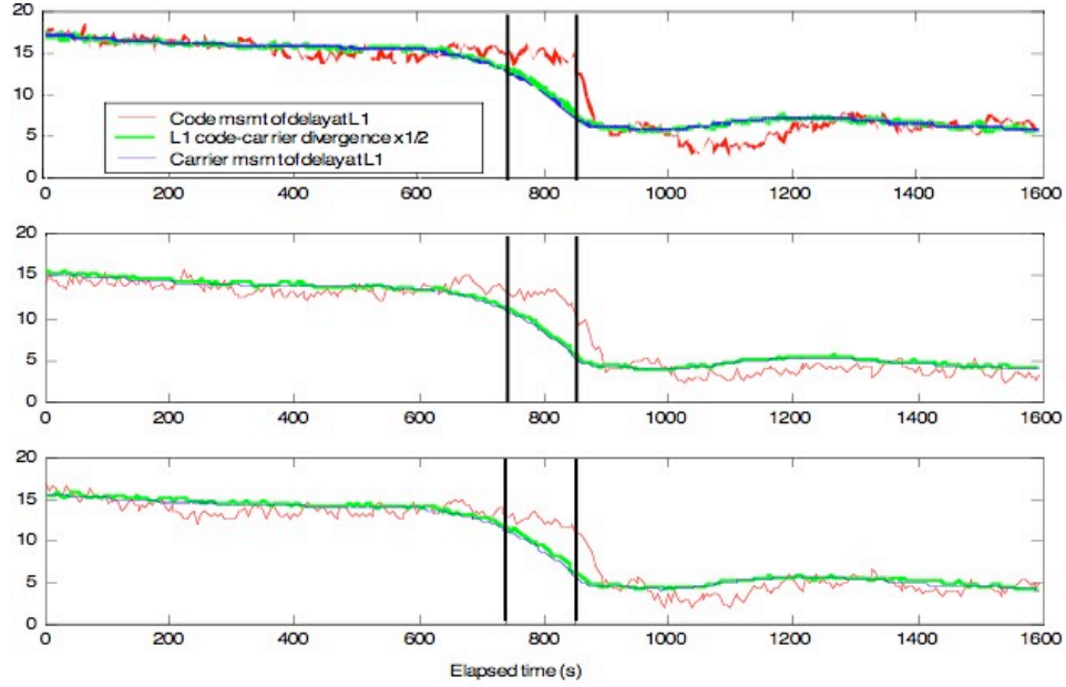
Figure 5.6: Slant ionospheric delay to SVN 40 from each receiver at Washington, D.C., WAAS station.
