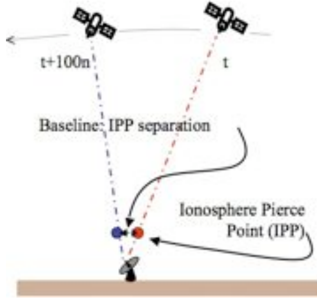
Figure 5.3: Illustration of the time step configuration.
