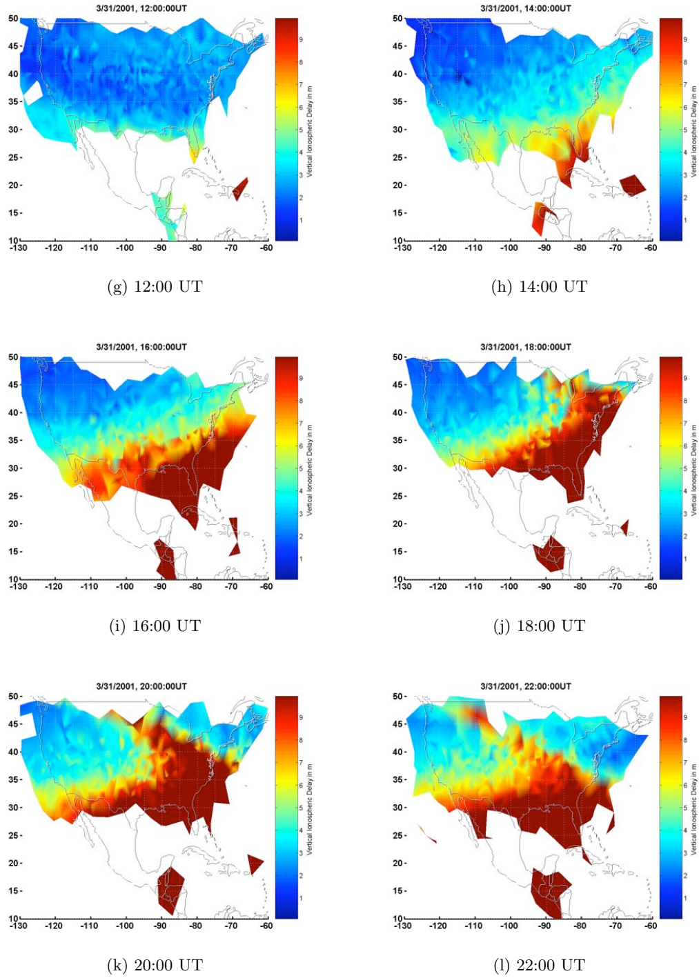
Figure B.5: 31 March 2001, 12:00–22:00 UT.
