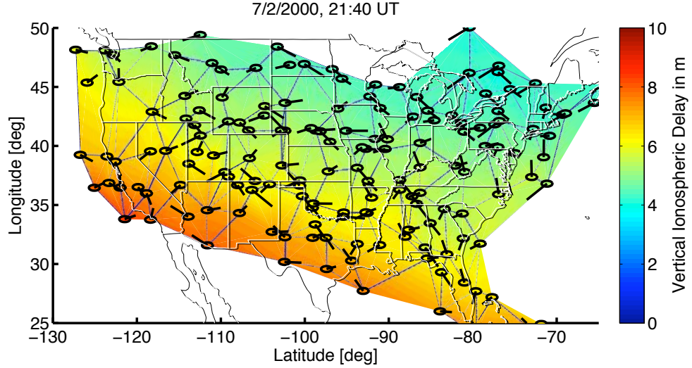
Figure 2.4: Contour map of nominal ionosphere over the United States. Colors range from 0 to 10 m of equivalent vertical range delay.
