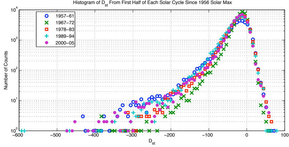
Figure 4.4: Histogram of 5 years post-solar-max for each solar cycle since 1957. The cycle whose max was in 1956 (blue) is underrepresented as there is no D_{st} data for 1956. The 2000–05 half-solar-cycle is plotted in magenta.
