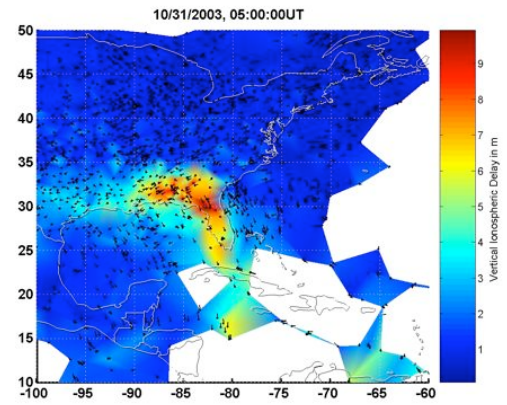
(f) 05:00 UT (31 October, 00:00 EST).
