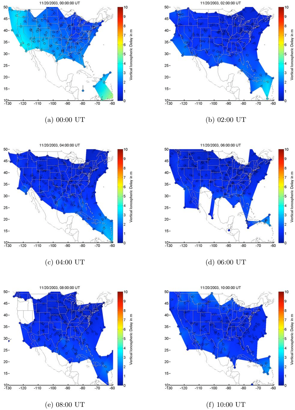
Figure B.11: 20 November 2003, 00:00–10:00 UT.
