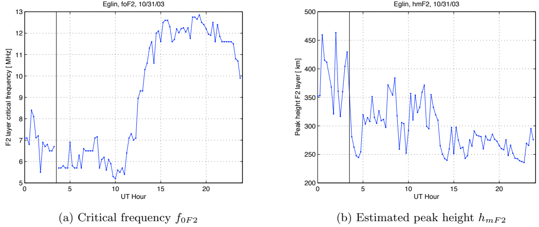
Figure 6.9: 31 October 2003, Eglin AFB ionosonde data.
