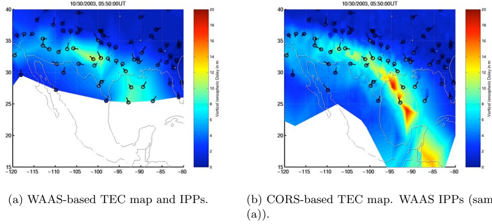
Figure 3.5: Comparison of ionosphere sampled at lower density by WAAS to “actual” activity, as observed in higher density CORS data, over the southern US on 30 October 2003.
