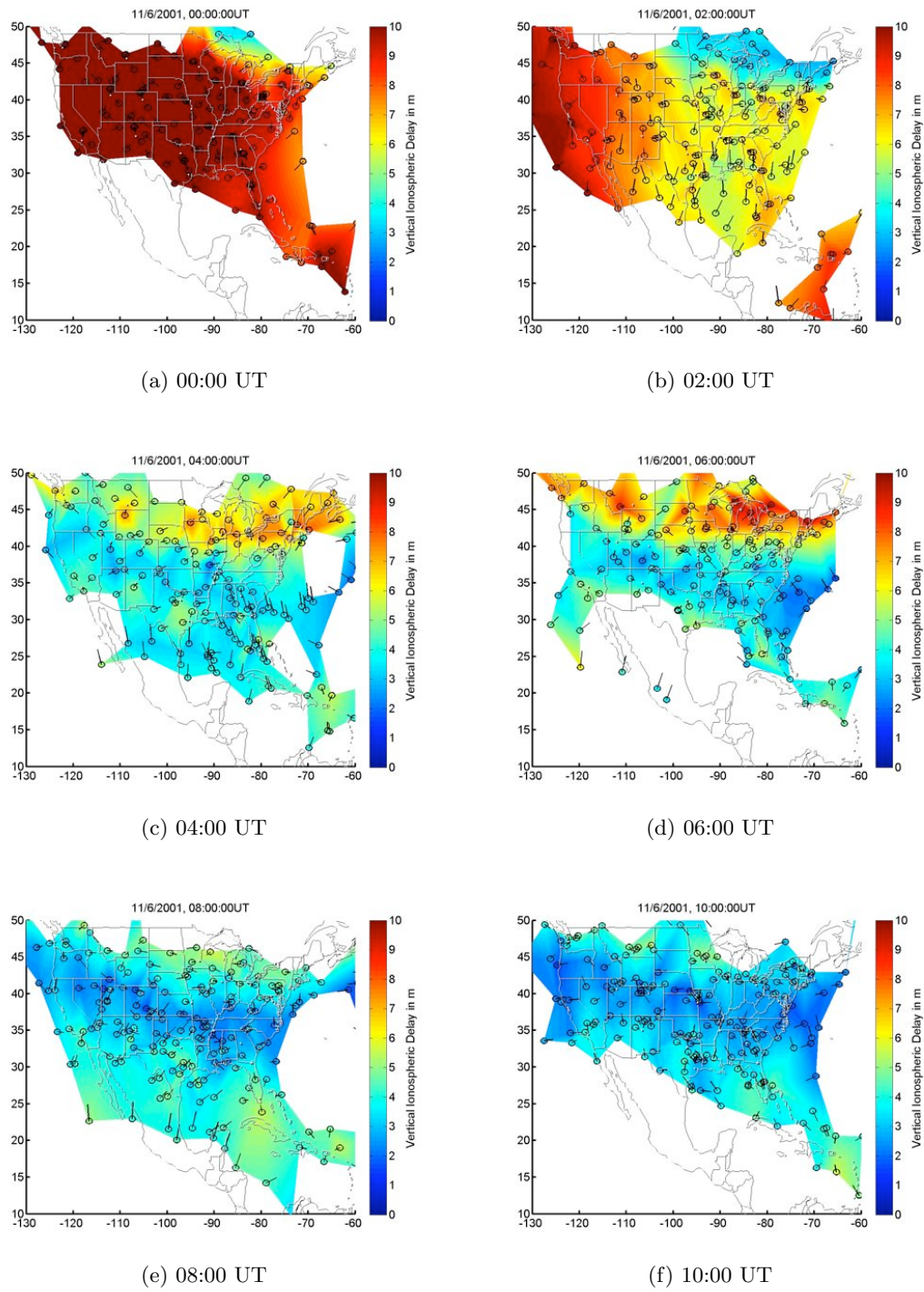
Figure B.7: 6 November 2001, 00:00–10:00 UT.
