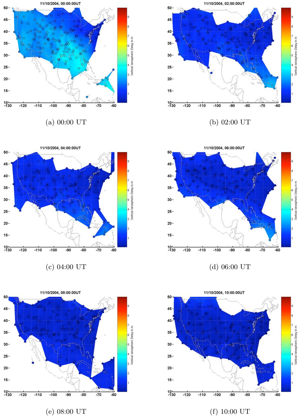
Figure B.14: 10 November 2004, 00:00–10:00 UT.
