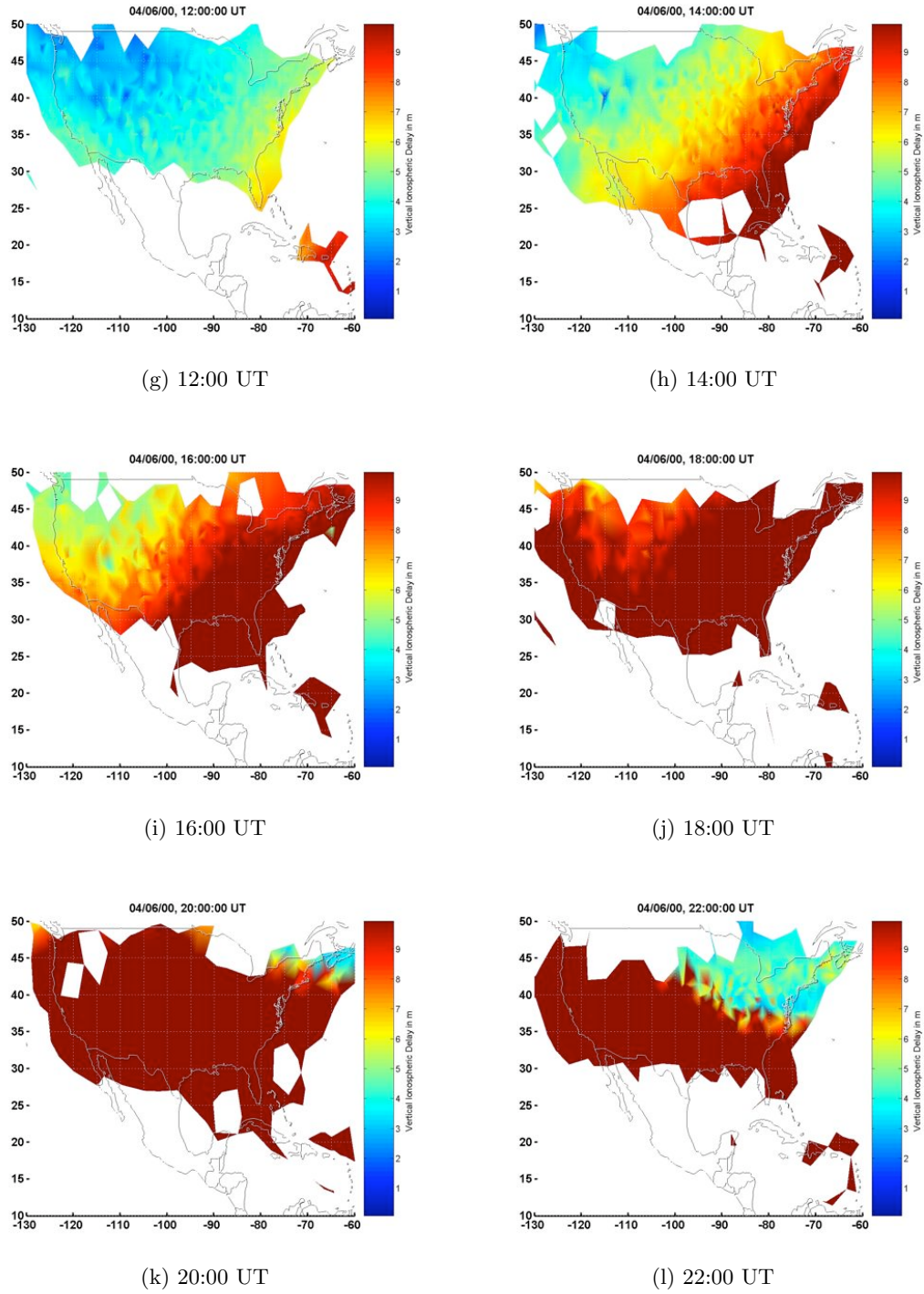
Figure B.1: 6 April 2000, 12:00–22:00 UT.
