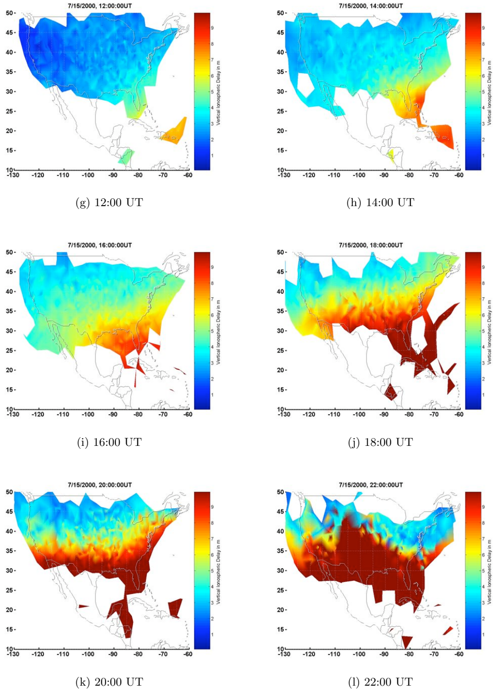
Figure B.3: 15 July 2000, 12:00–22:00 UT.
