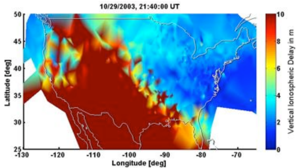
(b) Active
