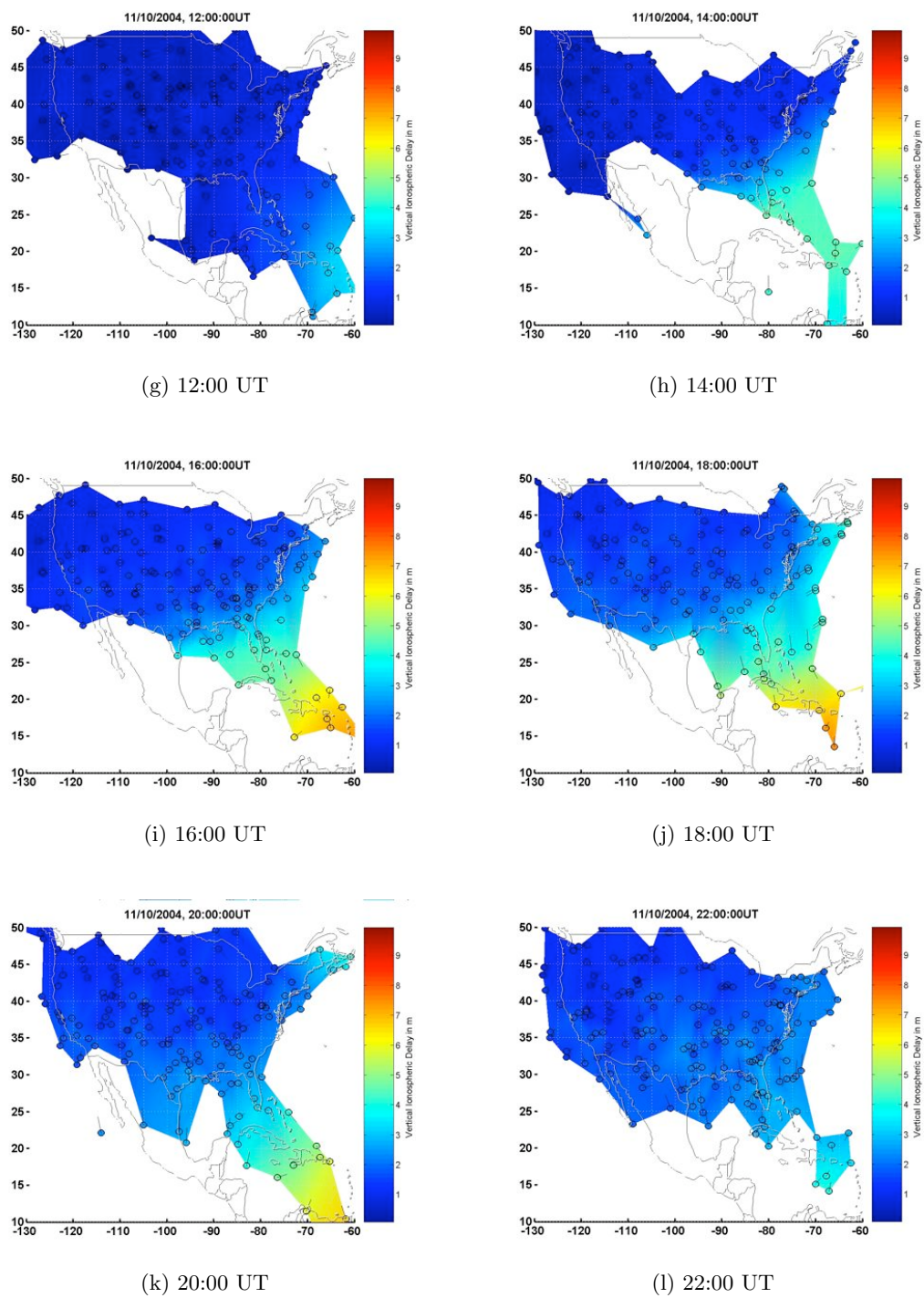
Figure B.14: 10 November 2004, 12:00–22:00 UT.
