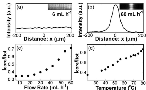
FIG. 2. (a) and (b) Plots of average intensity (arbitrary units, a.u.) of a digital micrograph taken of the light output of the water L^2 waveguide at the outlet of the microfluidic channel viewed through the transparent window for nonwaveguiding and waveguiding under various rates of flow and temperature settings. The insets show the digital micrographs used as the sources for the plots (data were smoothed prior to integration). In each case, the core was water at 21 ^{\circ}\text{C} and the cladding was water heated to 80 ^{\circ}\text{C} . Total rates of flow were 6 \text{mL h}^{-1} (a) and 60 \text{mL h}^{-1} (b), respectively. (c) Plot of intensity ratio ( I_{\text{core}}/I_{\text{total}} ) at the light output as a function of total flow rate ( T_{\text{core}}=21^{\circ}\text{C}, T_{\text{cladding}}=72^{\circ}\text{C} ). (d) Plot of intensity ratio ( I_{\text{core}}/I_{\text{total}} ) as a function of temperature in the cladding region (total rate of flow=60 \text{mL h}^{-1}, T_{\text{core}}=21^{\circ}\text{C} ). The error bars in both (c) and (d) were smaller than the size of the symbols.
