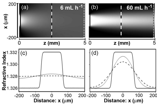
FIG. 3. Simulated two-dimensional ( xz ) distributions of refractive index in a 5 mm long waveguide formed by water at total rates of flow of 6 \text{ mL h}^{-1} (a) and 60 \text{ mL h}^{-1} (b), and T_{\text{core}}=21 \text{ }^\circ\text{C} and T_{\text{cladding}}=72 \text{ }^\circ\text{C} . Plot of the refractive index as a function of distance from the center of the waveguide in the transverse ( x ) direction for three positions along a waveguide (in z direction)—i.e., the beginning (solid line), the middle (dashed line), and the end (dotted line) of the channel at total rates of flow of 6 \text{ mL h}^{-1} (c) and 60 \text{ mL h}^{-1} (d). The residence times are 0.12 s in (a) and 0.012 s in (b), respectively.
