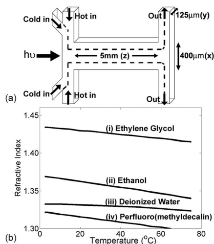
FIG. 1. (a) Schematic diagram of the microfluidic channel used for thermally generated optical waveguides. The length, width, and height of the channel are 5 mm, 400 \mu\text{m} , and 125 \mu\text{m} , respectively. The dotted line shows the boundary between hot and cold liquids under laminar flow conditions. (b) Graph of refractive indices measured using benchtop Bausch and Lomb refractometer as a function of temperature for: (i) ethylene glycol, (ii) ethanol, (iii) deionized water, and (iv) perfluoro(methyldecalin). The average slopes or TO coefficients ( dn_D/dT, K^{-1} ) are -2.6 \times 10^{-4} (ethylene glycol), -4.0 \times 10^{-4} (ethanol), -1.2 \times 10^{-4} (water), and -3.4 \times 10^{-4} [perfluoro(methyldecalin)], respectively.
