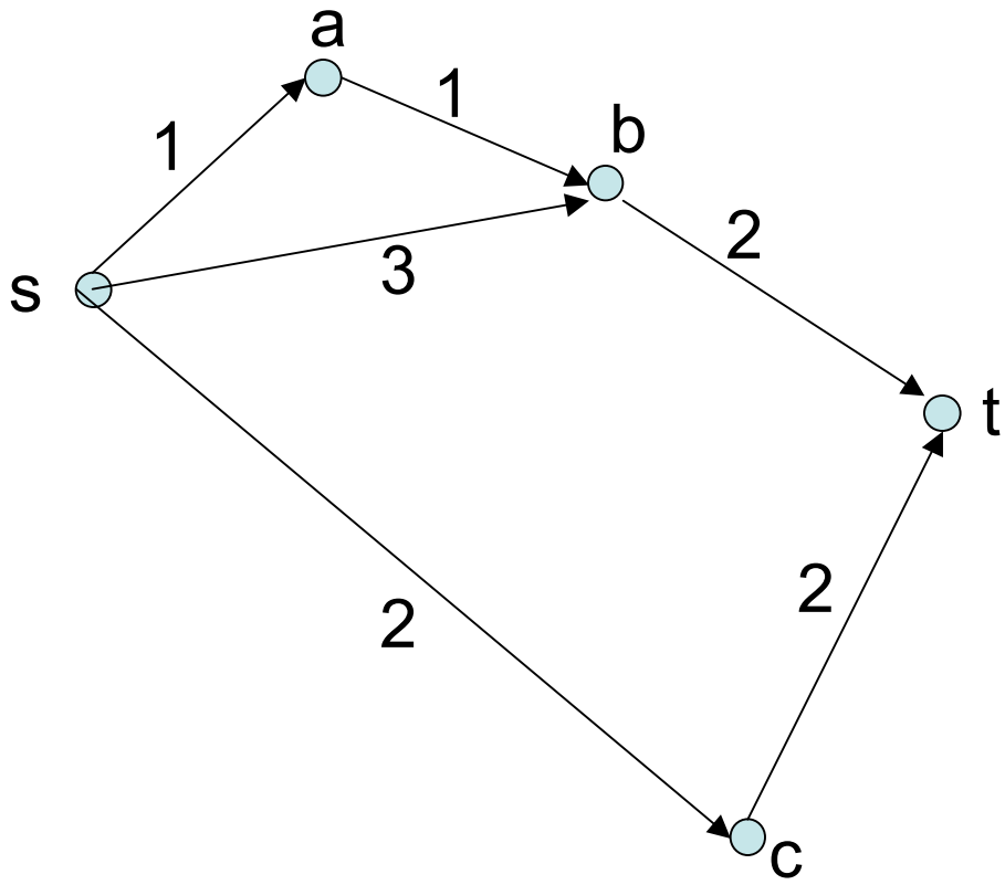
Graph for problem 1. The numbers on edges denote costs.
