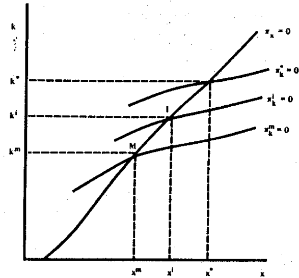
Figure 3.4. For \pi_{Xk} .
