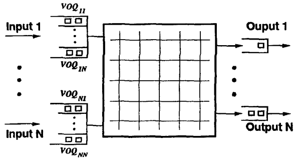
Fig. 1. A CIOQ switch
