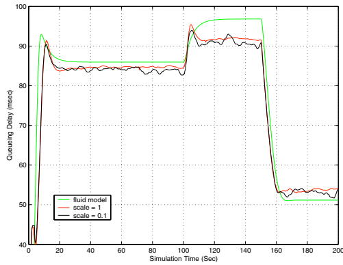
Fig. 7. With slower links: Average queuing delay at Q1
