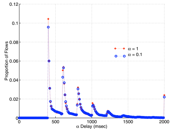
Fig. 18. Histogram of normalized delays of grp2 flows (DropTail).
