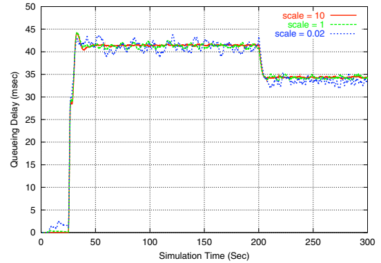
Fig. 9. In a more complex network: Average queuing delay at R1-R5
