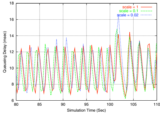
Fig. 6. With faster links: Average queuing delay at Q1 (zoomed in)
