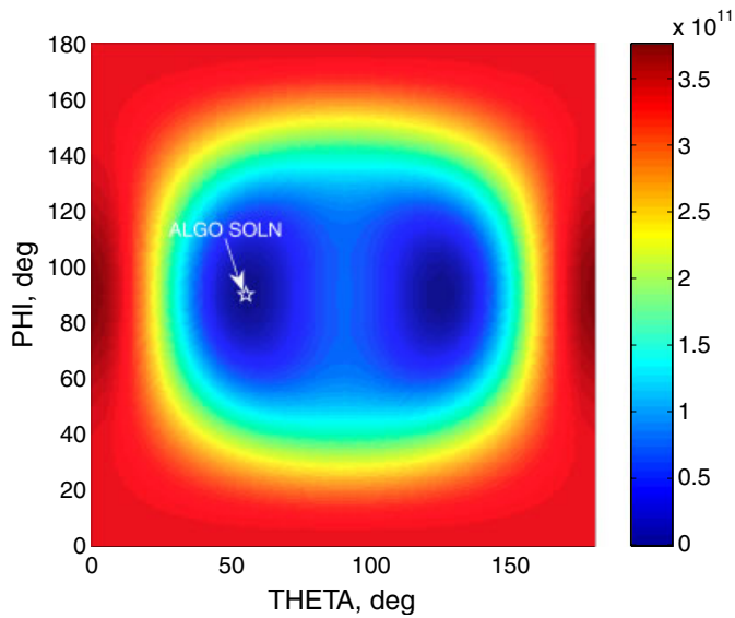
Figure 6. Profile of the determinant of the acoustic tensor for three-invariant model with \rho=0.7 at onset of localization.
