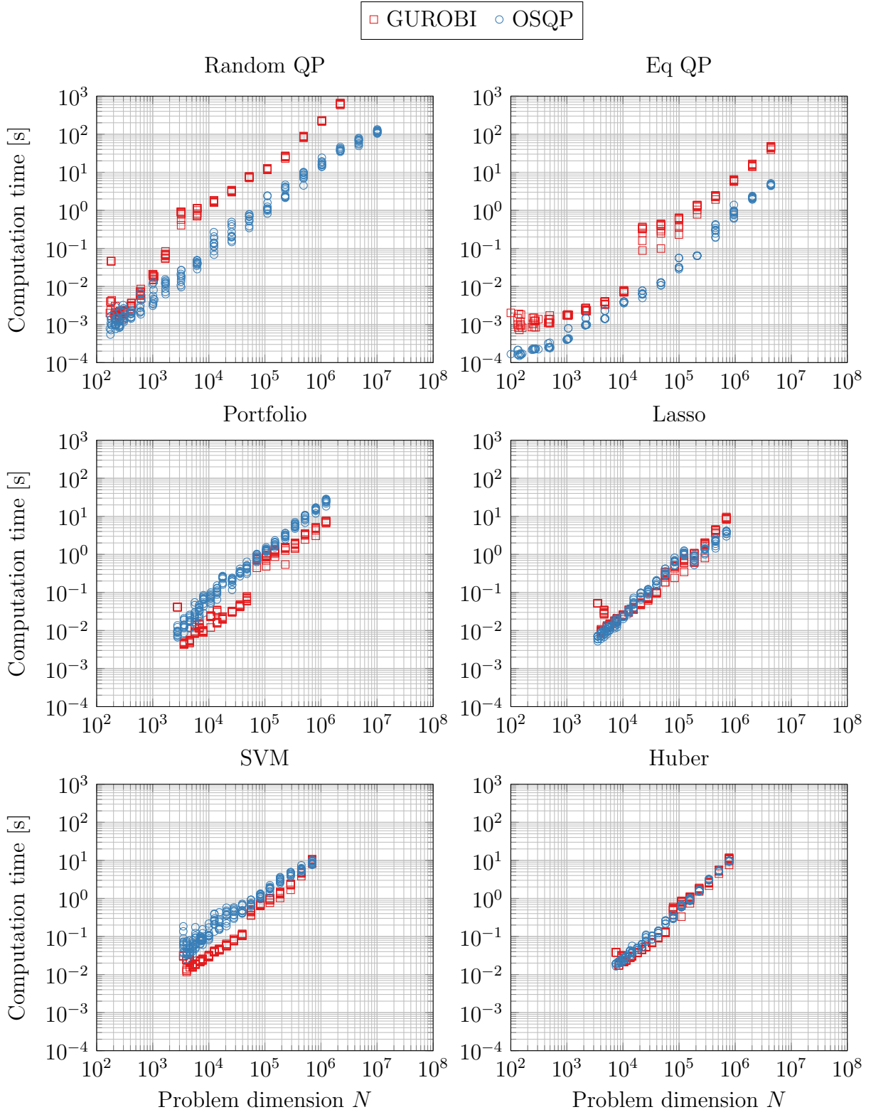
Figure 2: Computation time vs problem dimension for OSQP and GUROBI for high accuracy mode.
