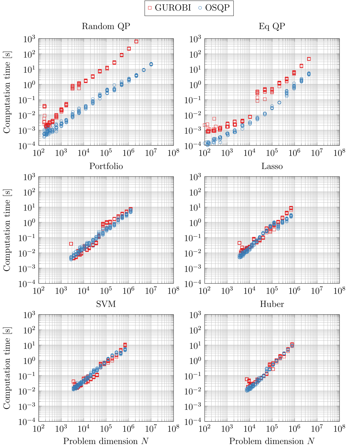
Figure 1: Computation time vs problem dimension for OSQP and GUROBI for low accuracy mode.
