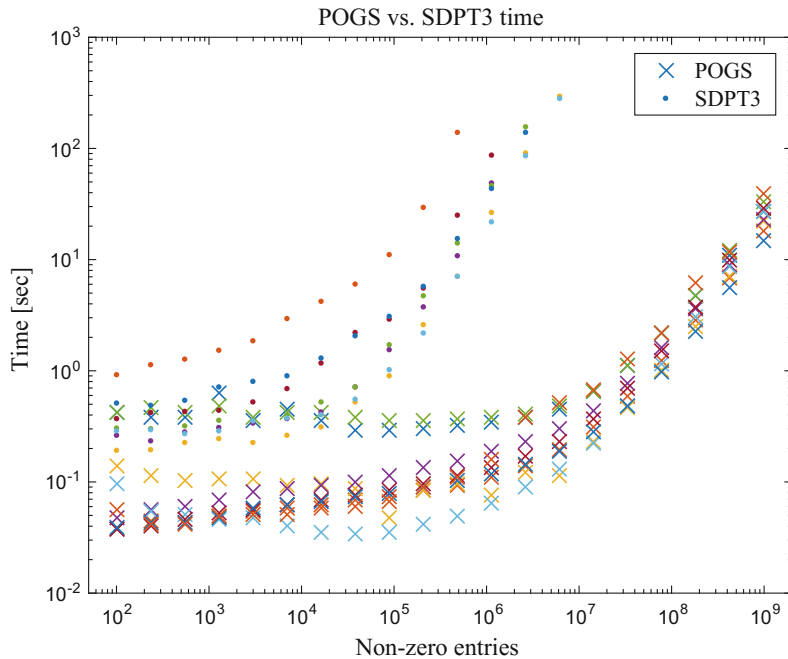
Fig. 4.1 POGS (GPU version) versus SDPT3 for dense matrices (color represents problem class)
