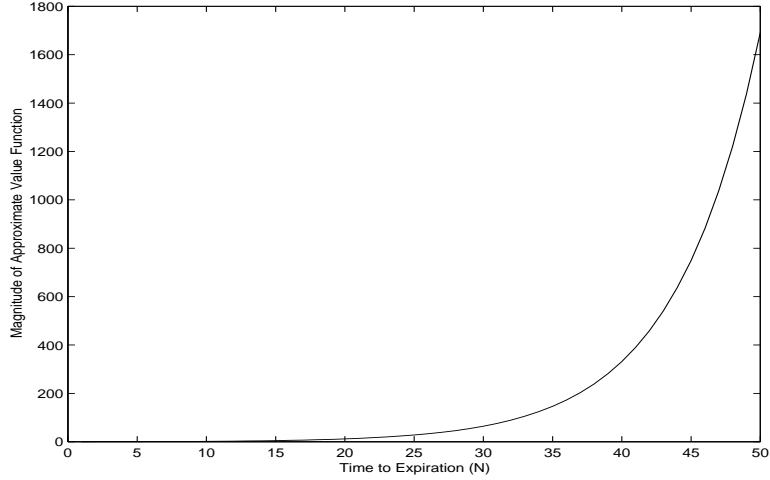
Figure 1: Exponential growth of the error in the example of Section 4.2.
