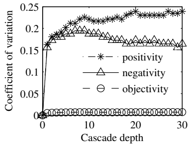
Figure 5: Coefficient of variation ( \sigma/\mu ) of relative-to-baseline positivity, negativity, and objectivity. The values are calculated within nodes of a particular cascade at a given cascade depth, L , averaged over all cascades.
