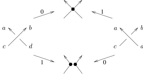
FIGURE 2. The top picture represents the singularization of a crossing, and the bottom picture the smoothing. The smoothing and the singularization are also called the 0- and 1-resolutions of the crossing; which is which depends on whether the original crossing is positive or negative, as shown in the figure.
