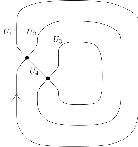
FIGURE 10. A total braid graph.
