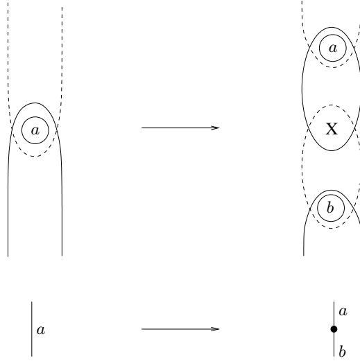
FIGURE 6. An insertion along an edge changes the planar Heegaard diagram as shown here.
