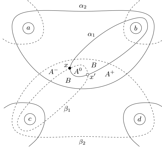
FIGURE 4. The planar diagrams at a crossing.
