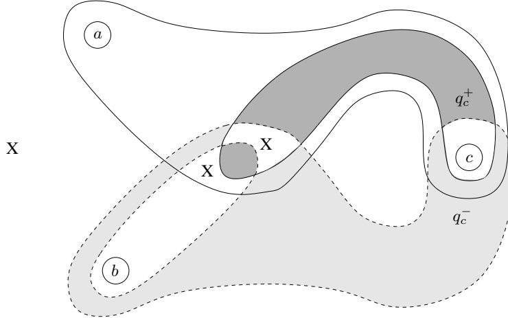
FIGURE 5. This is a planar Heegaard diagram for an unlink S , obtained as follows: start with a planar projection of the unknot having a single crossing, smooth that crossing, and apply the procedure in Section 2.1. In the diagram, we show the periodic domain \pi_1 = \pi_+(c) - \pi_-(c) by indicating multiplicity +1 by darker shading, and multiplicity -1 by lighter shading.
