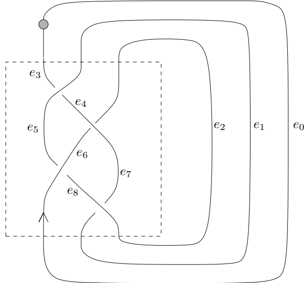
FIGURE 1. A decorated braid projection for the figure-eight knot. The gray dot marks the subdivision of the distinguished edge.
