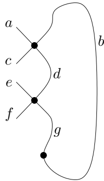
FIGURE 3. A partial braid graph with four exterior edges and three vertices.
