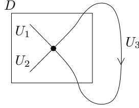
FIGURE 8. A partial braid graph with one crossing. We write the corresponding U variable on each edge.
