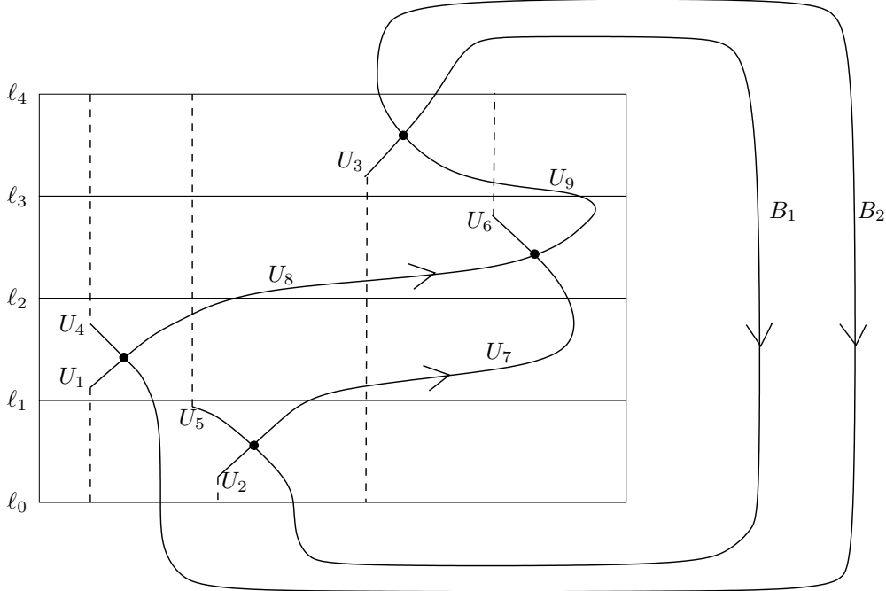
FIGURE 9. The square D is partitioned into strips and has the dashed curves added. On each edge we mark a corresponding variable.
