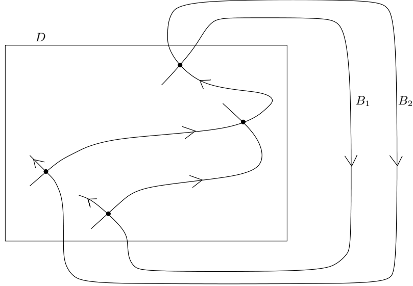
FIGURE 7. A partial braid graph and its closure. Here n = 5 and k = 2 . The closure \hat{\Gamma} has six loose ends, four crossings, and no two-valent vertices.
